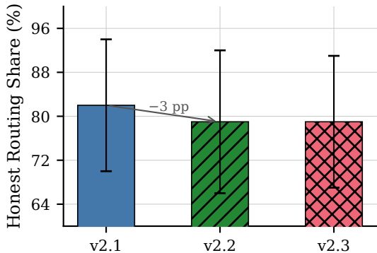
Fig. 6 — Honest Routing by Version (Collusion Ring, N=50 , 20 seeds)
