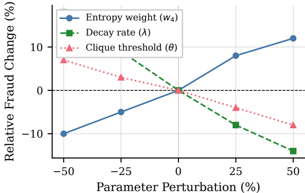
Fig. 7 — Sensitivity Analysis (Collusion Ring, N=50 , 5 seeds)
