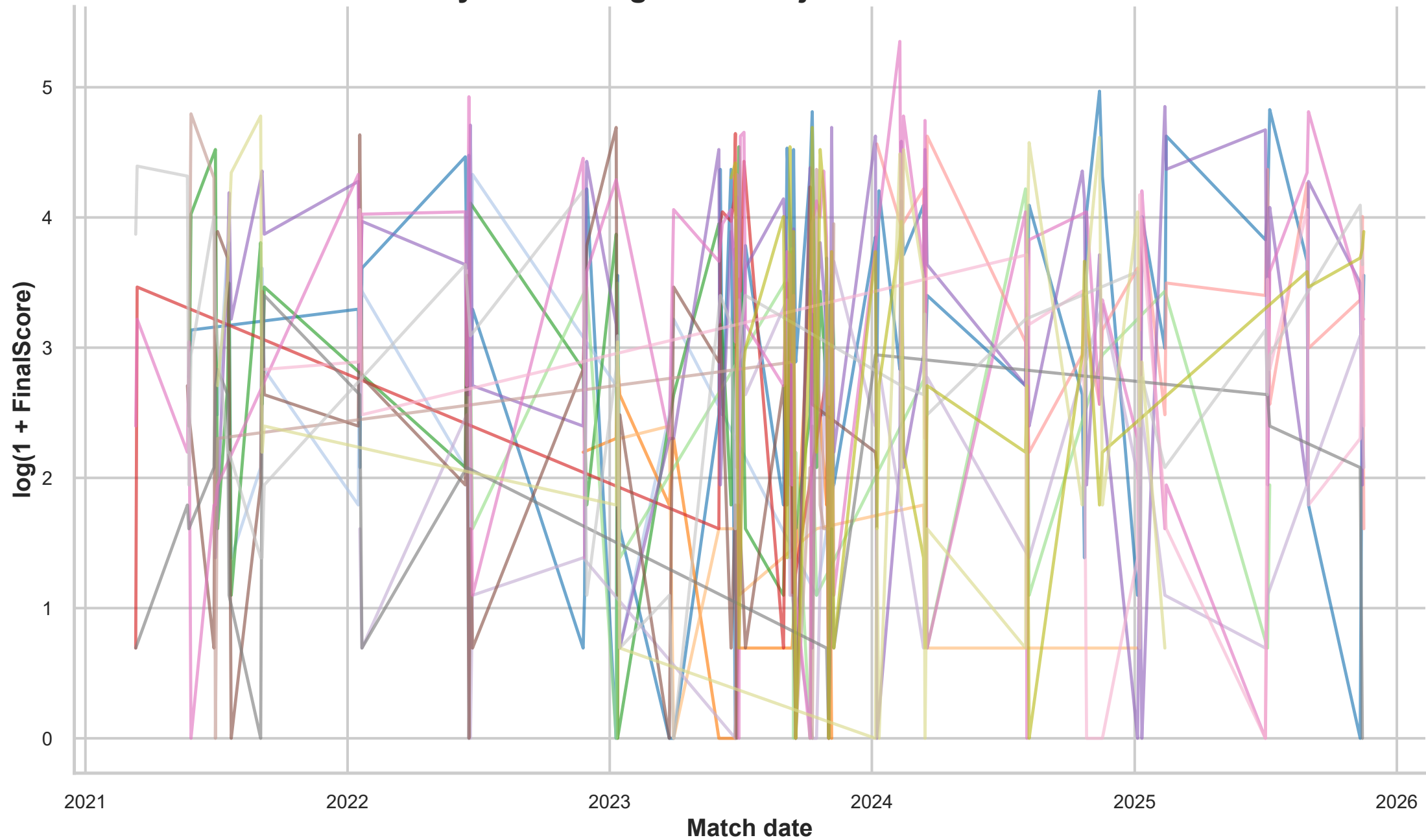
Player-wise Log-Score Trajectories Over Time
