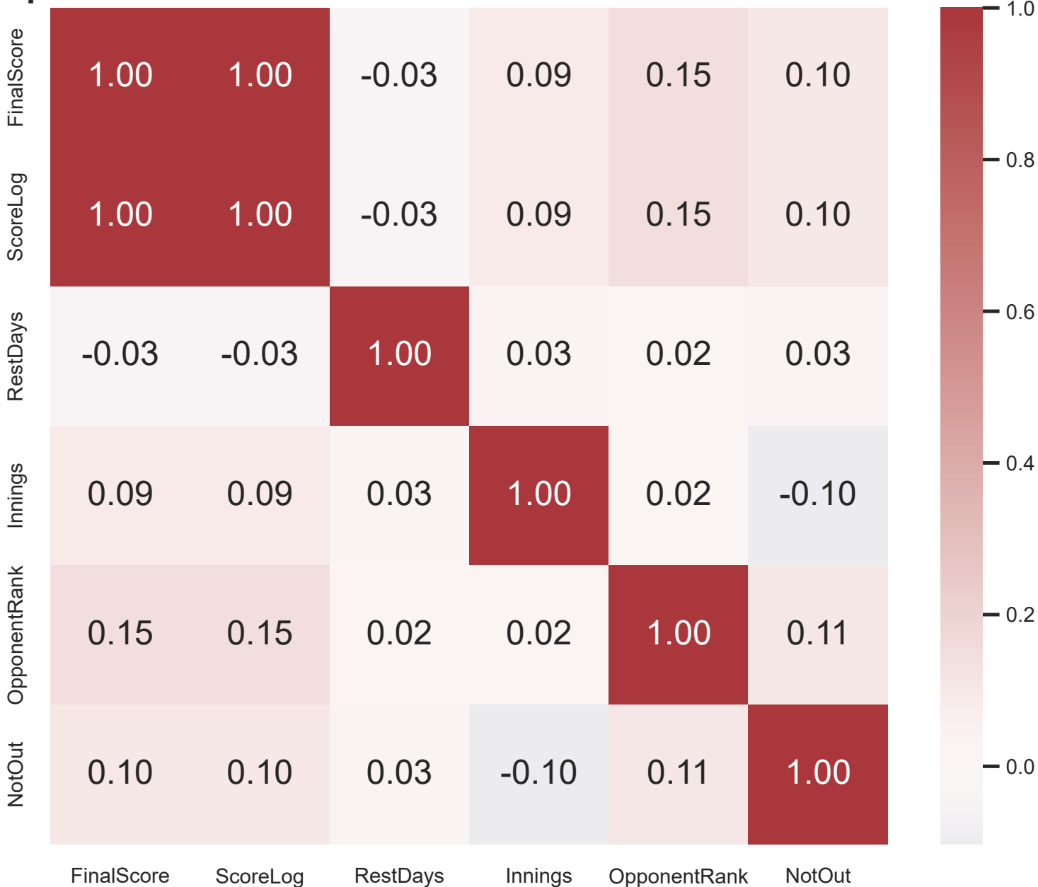
Spearman Correlation Matrix for Numeric Model Variables
