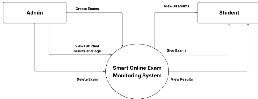
Figure 3.1.5 DFD Diagram
