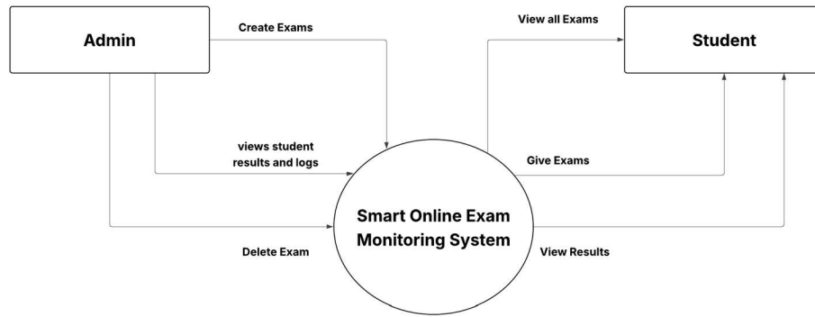
Figure 3.1.5 DFD Diagram
