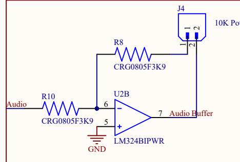
Audio buffer
