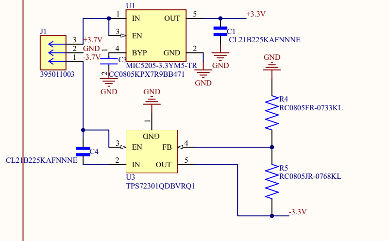
Voltage regulation
