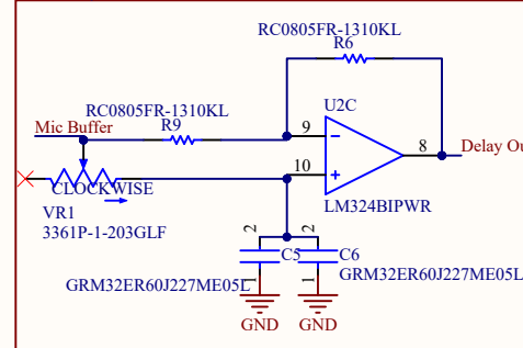
Noise delay
