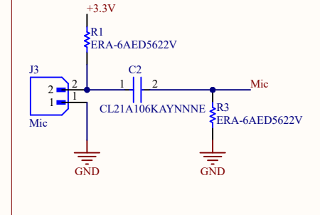
Microphone biasing
