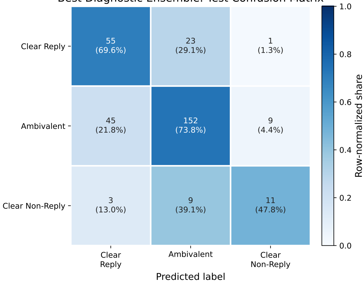
Best Diagnostic Ensemble: Test Confusion Matrix
