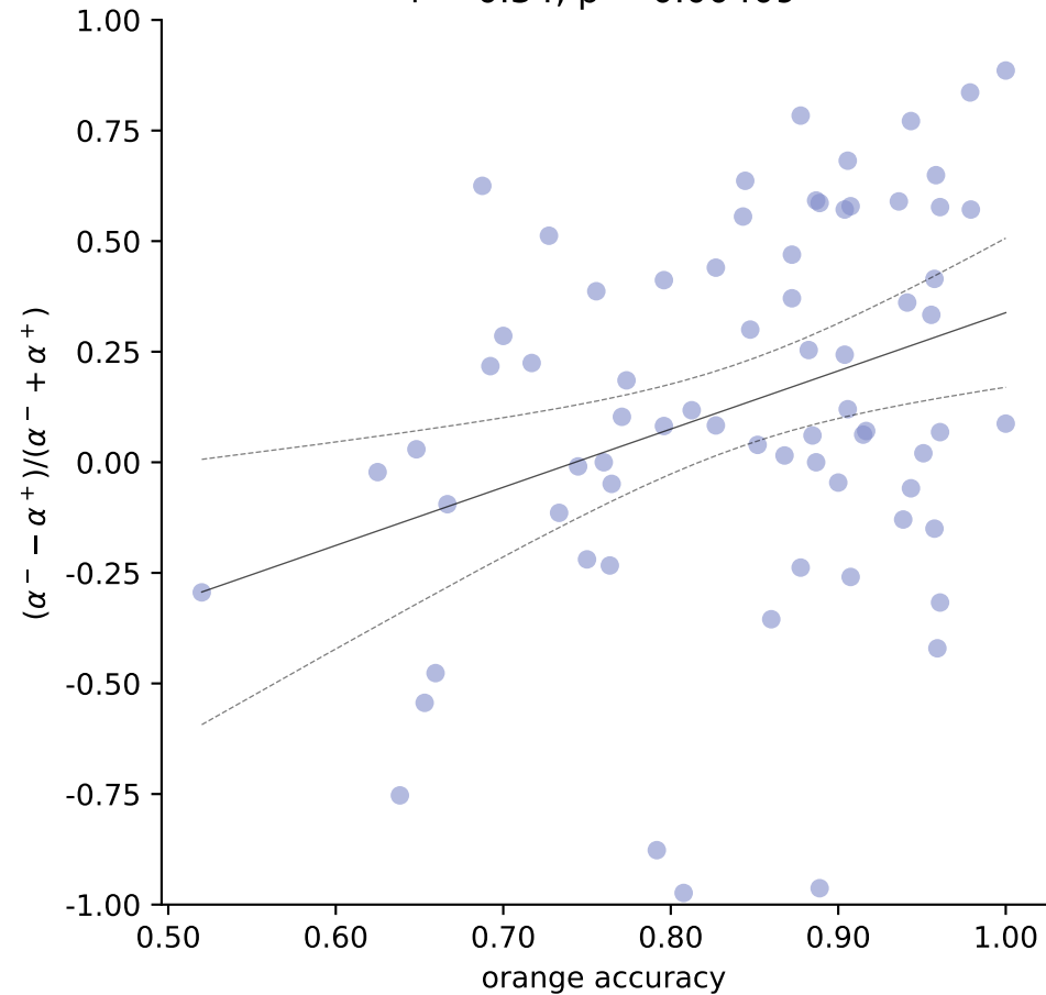
RSTD ratio vs orange accuracy r = 0.34, p = 0.00409
