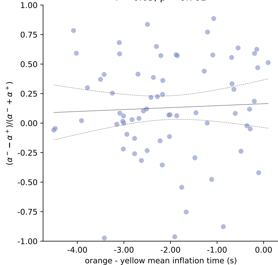
RSTD ratio vs orange - yellow mean inflation time r = 0.05 , p = 0.702
