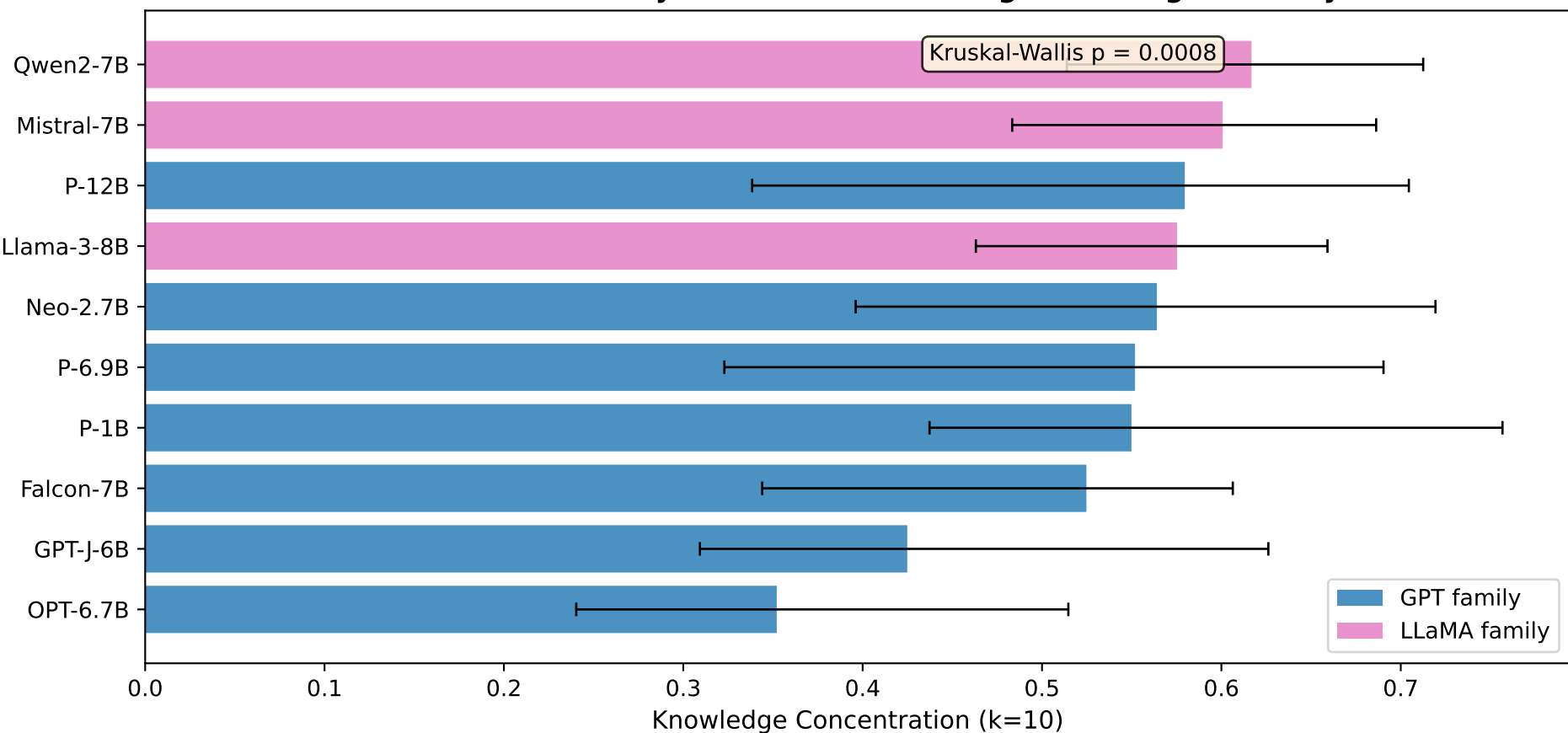
Architecture Family Determines Knowledge Encoding Efficiency
