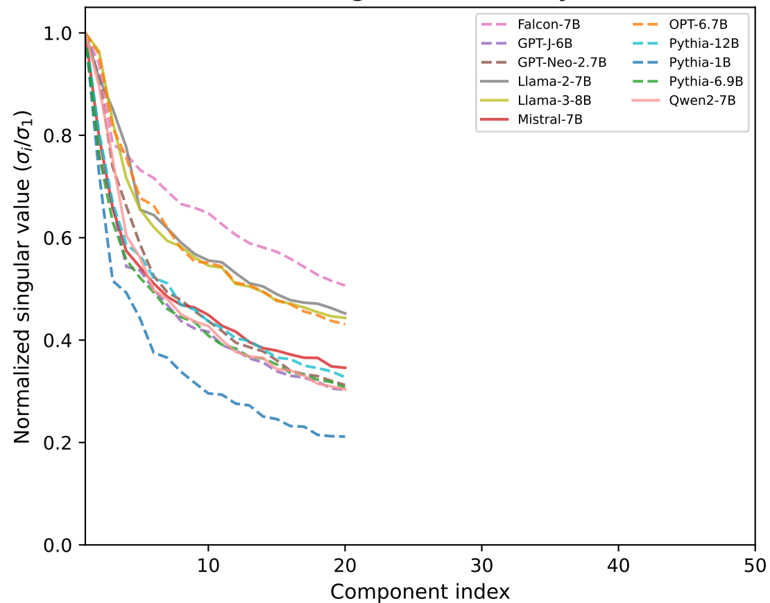
(a) Singular value decay
