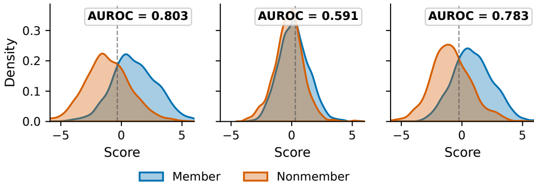
Mixed-data SAE
