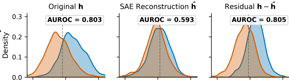
Member-only SAE
