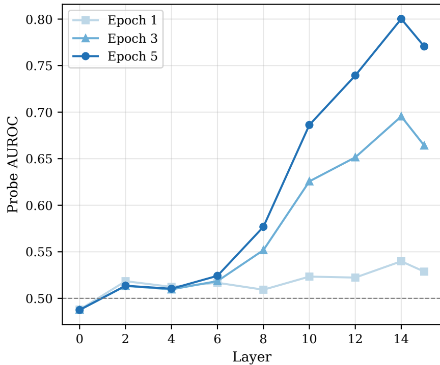
(b) Membership probe
