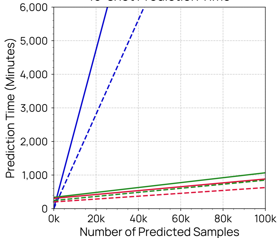
10-shot Prediction Time
