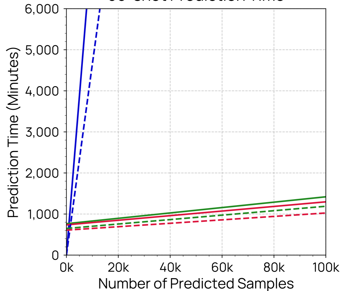
50-shot Prediction Time
