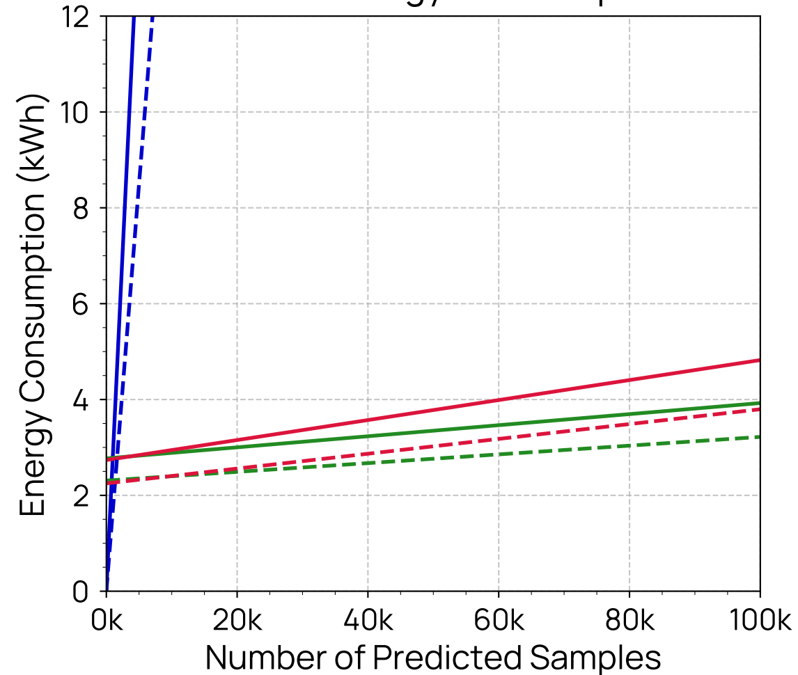
50-shot Energy Consumption
