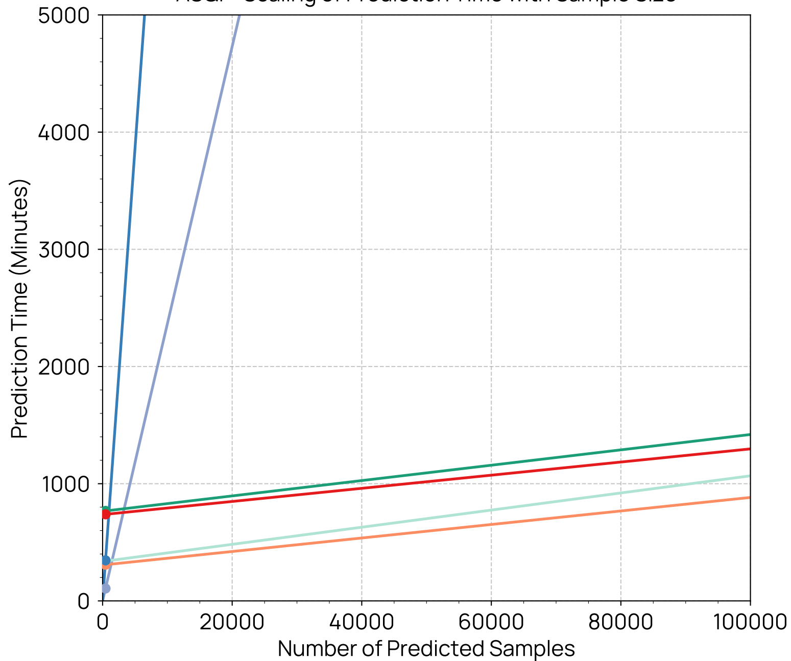
TASD: Scaling of Prediction Time with Sample Size
