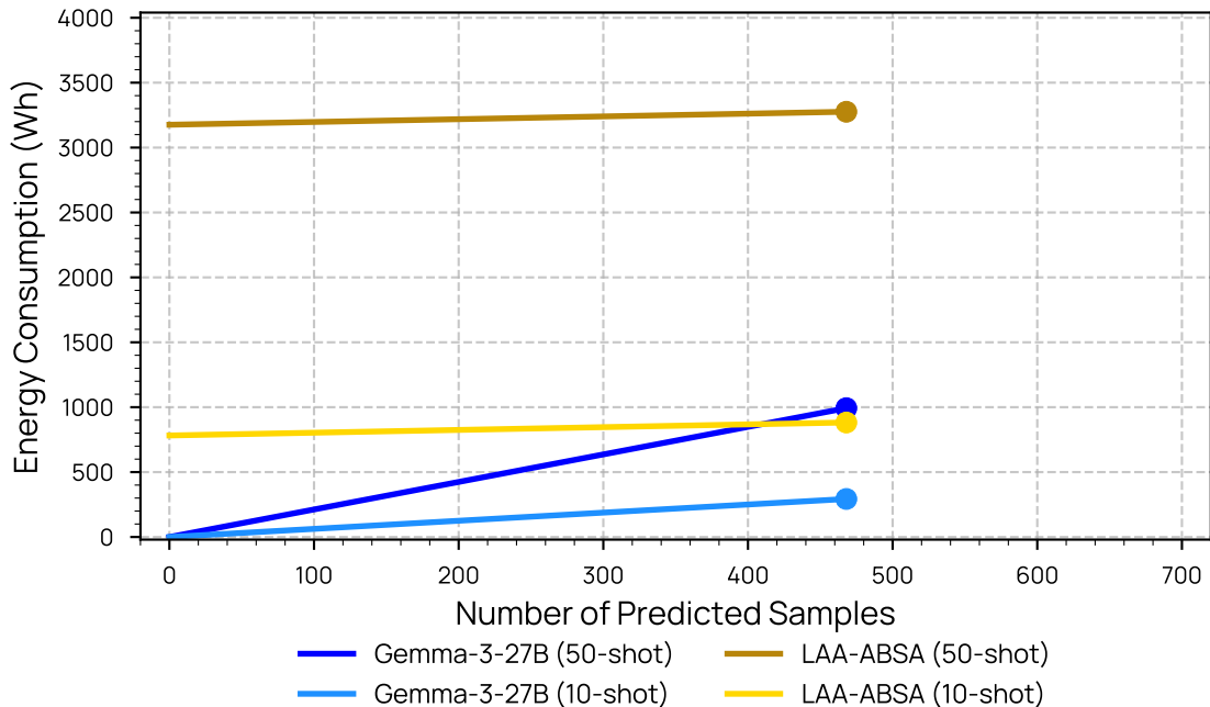
TASD: Energy Consumption vs. Number of Predicted Samples
