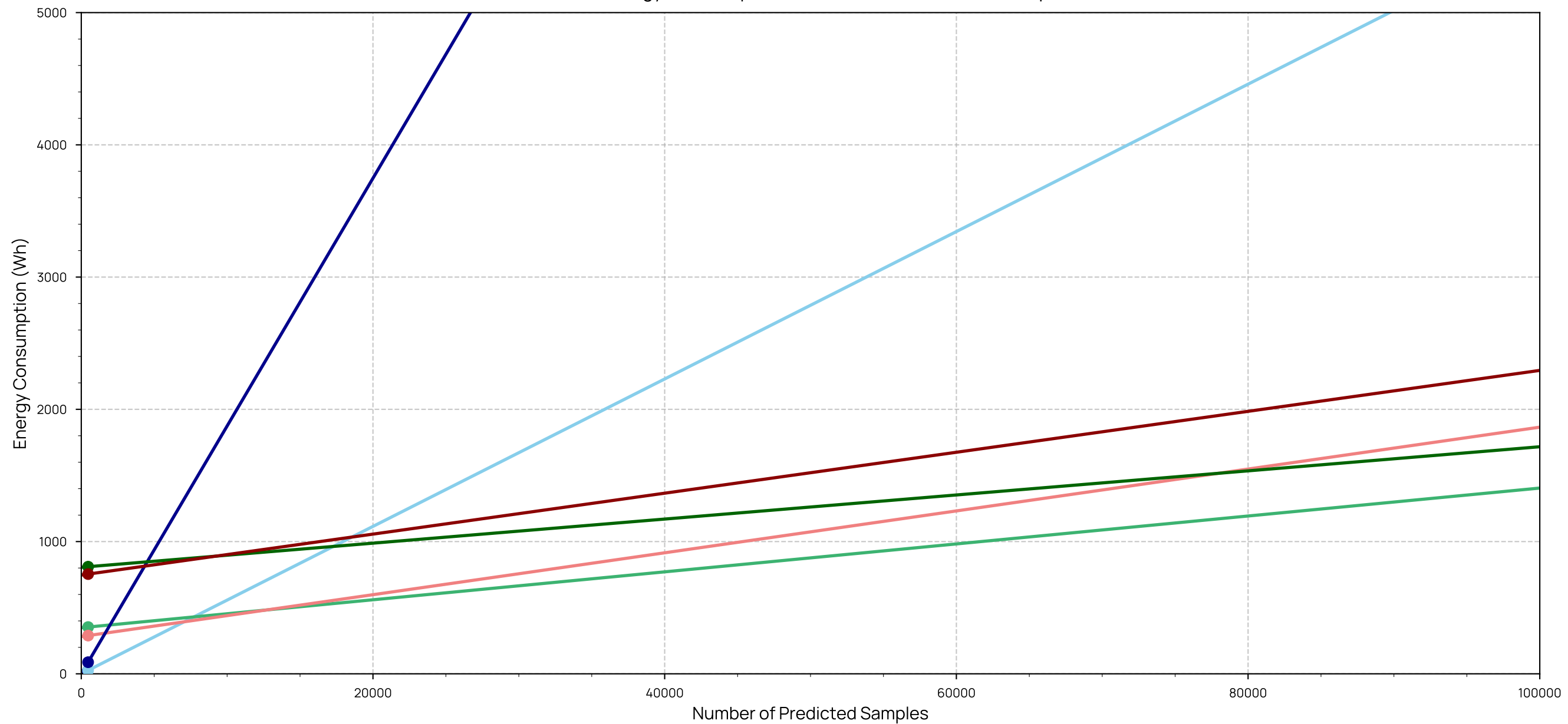
TASD: Energy Consumption vs. Number of Predicted Samples
