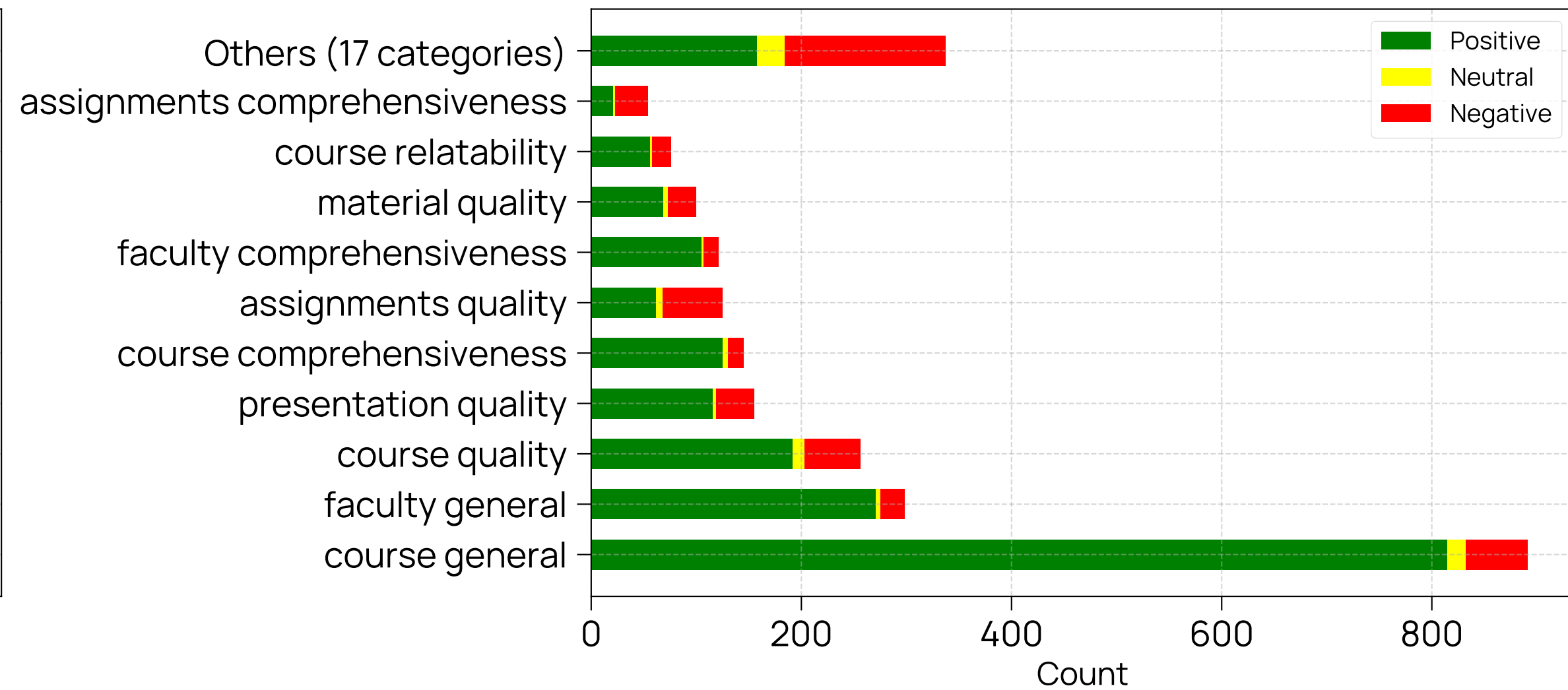
Coursera - ASQP
