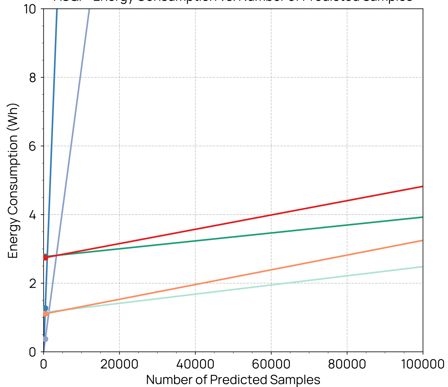
TASD: Energy Consumption vs. Number of Predicted Samples
