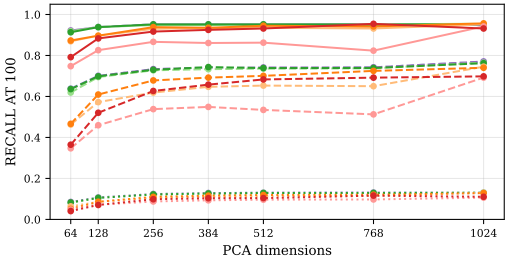
Retrieval RECALL AT 100 by Dimension
