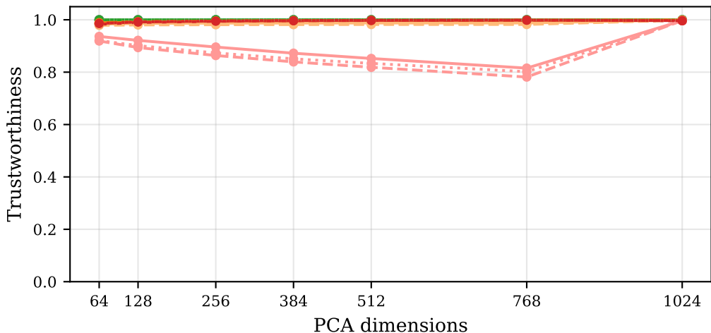
Trustworthiness vs. Dimension (k=20)
