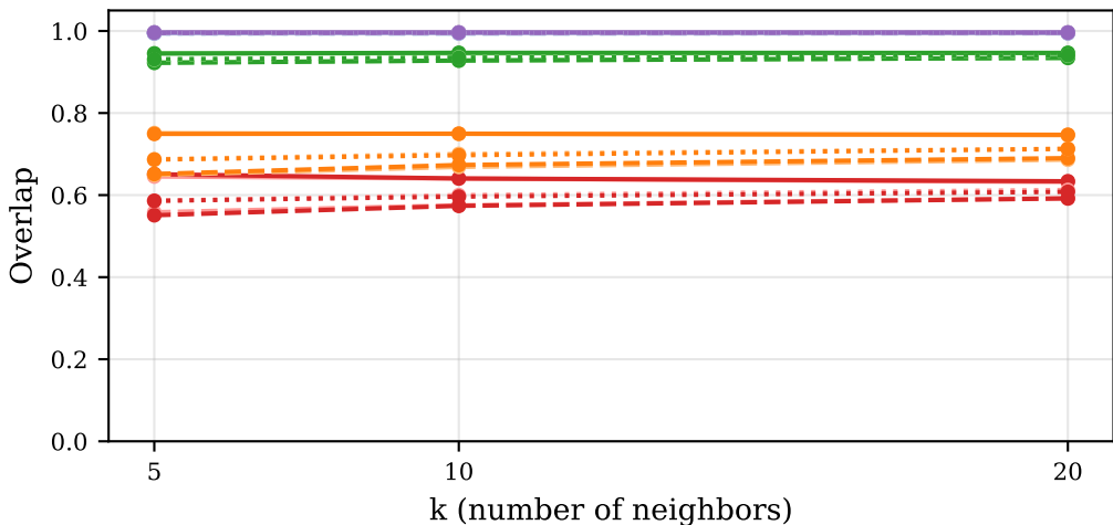
Overlap (d=1024)
