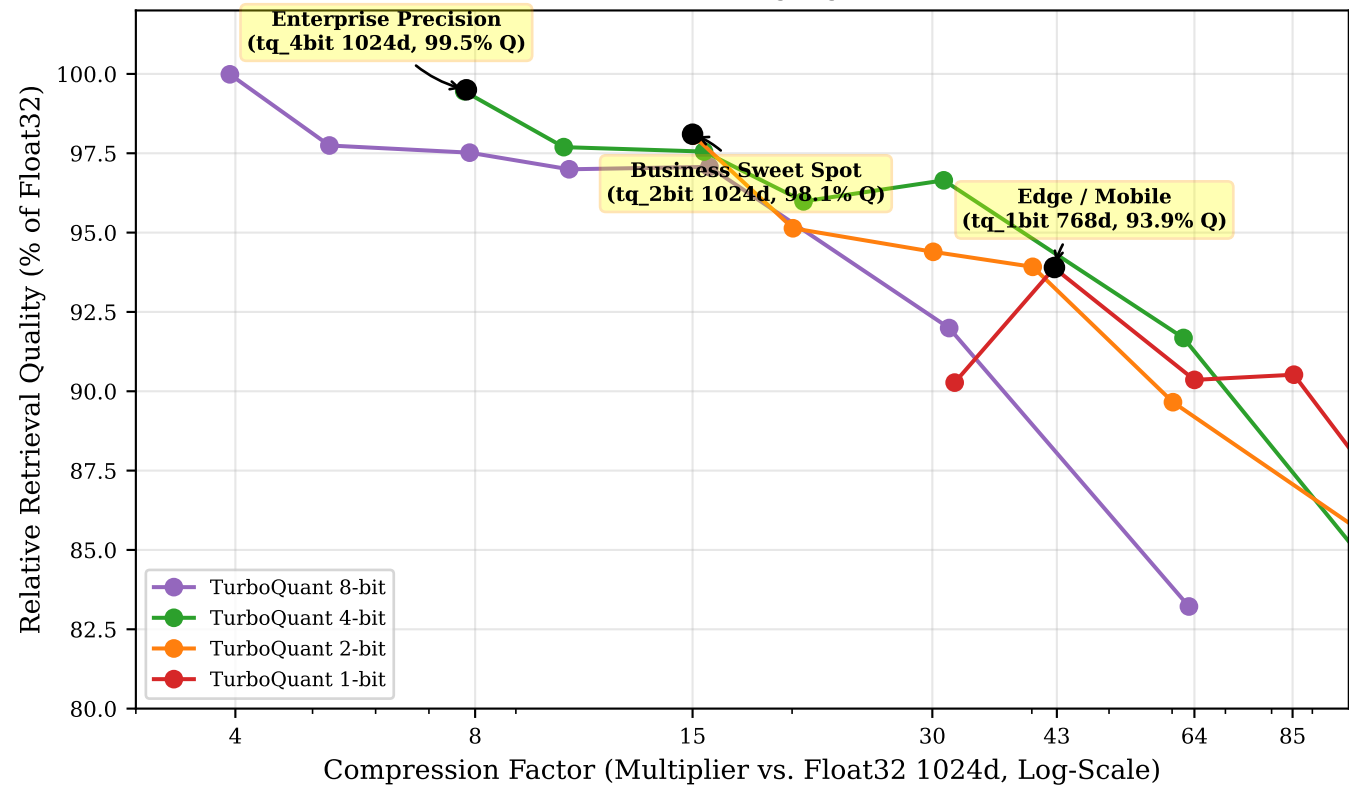
TurboQuant Trade-off Space with Highlighted Application Scenarios
