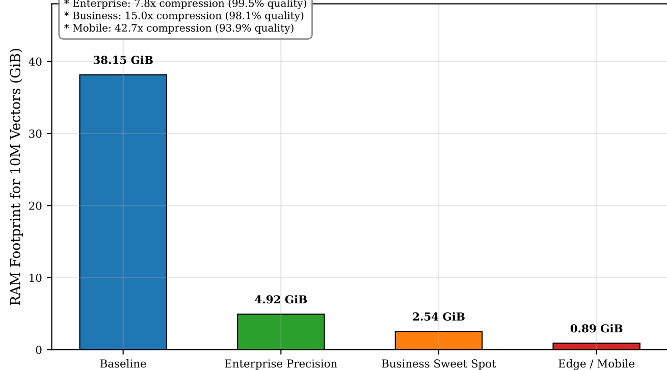
Memory Footprint Comparison across Application Scenarios (10M Vectors)
