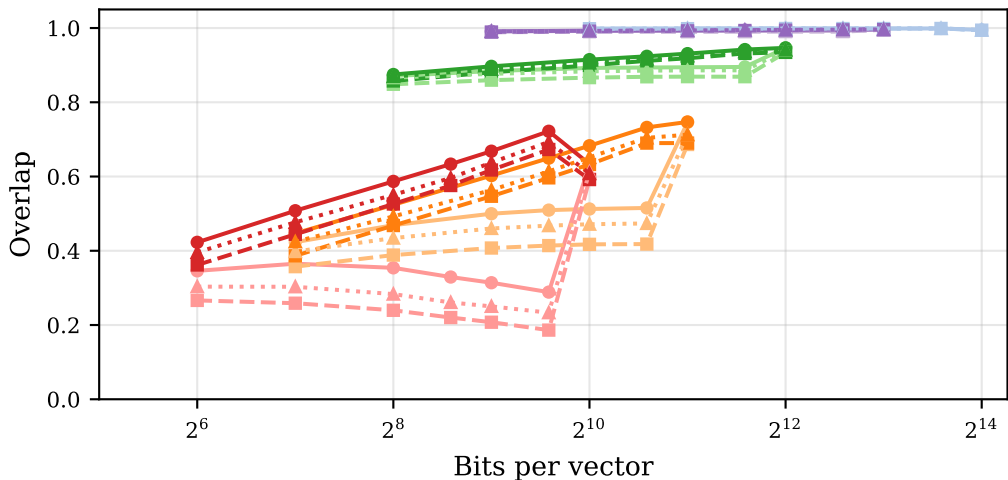
Overlap vs. Compression (k=20)
