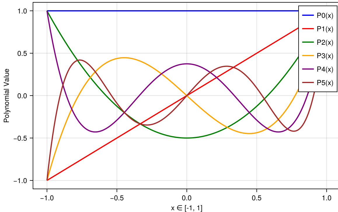
Legendre Polynomials P_0(x) to P_5(x)
