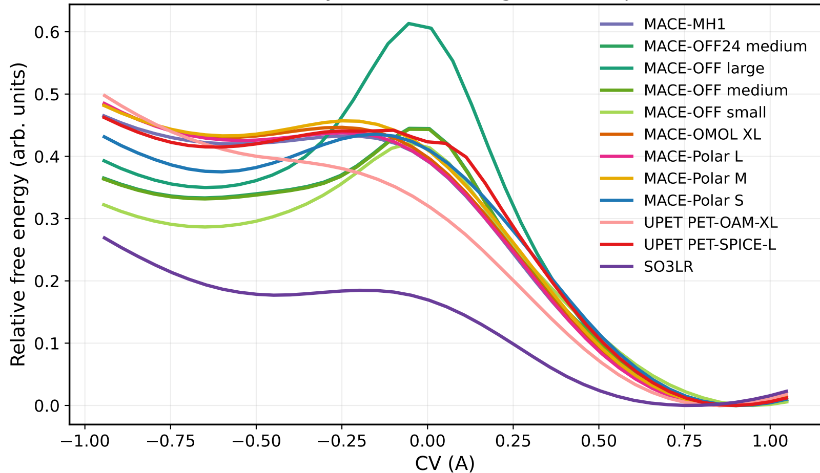
f-malonaldehyd: umbrella integration comparison
