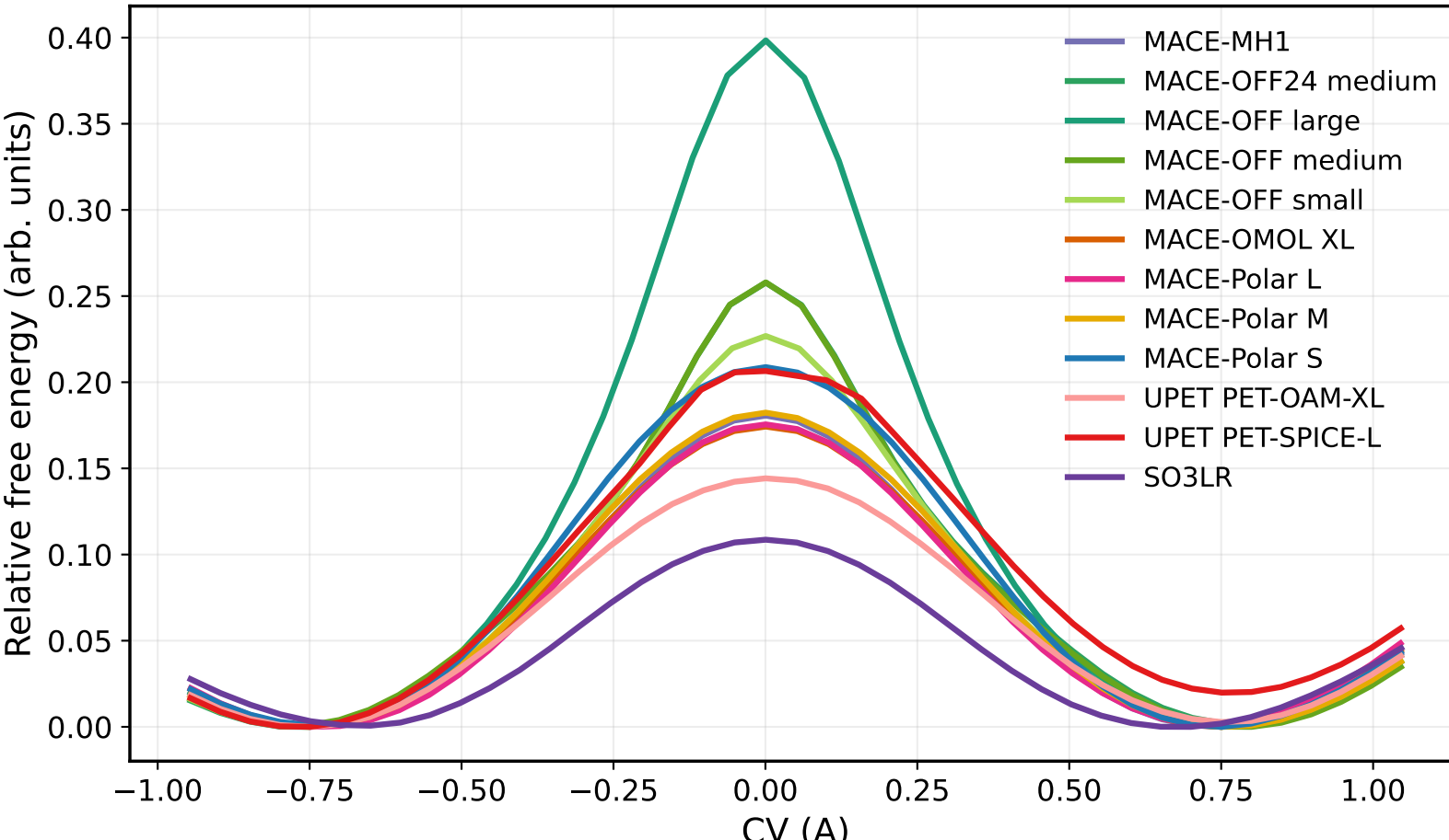
malonaldehyd: umbrella integration comparison
