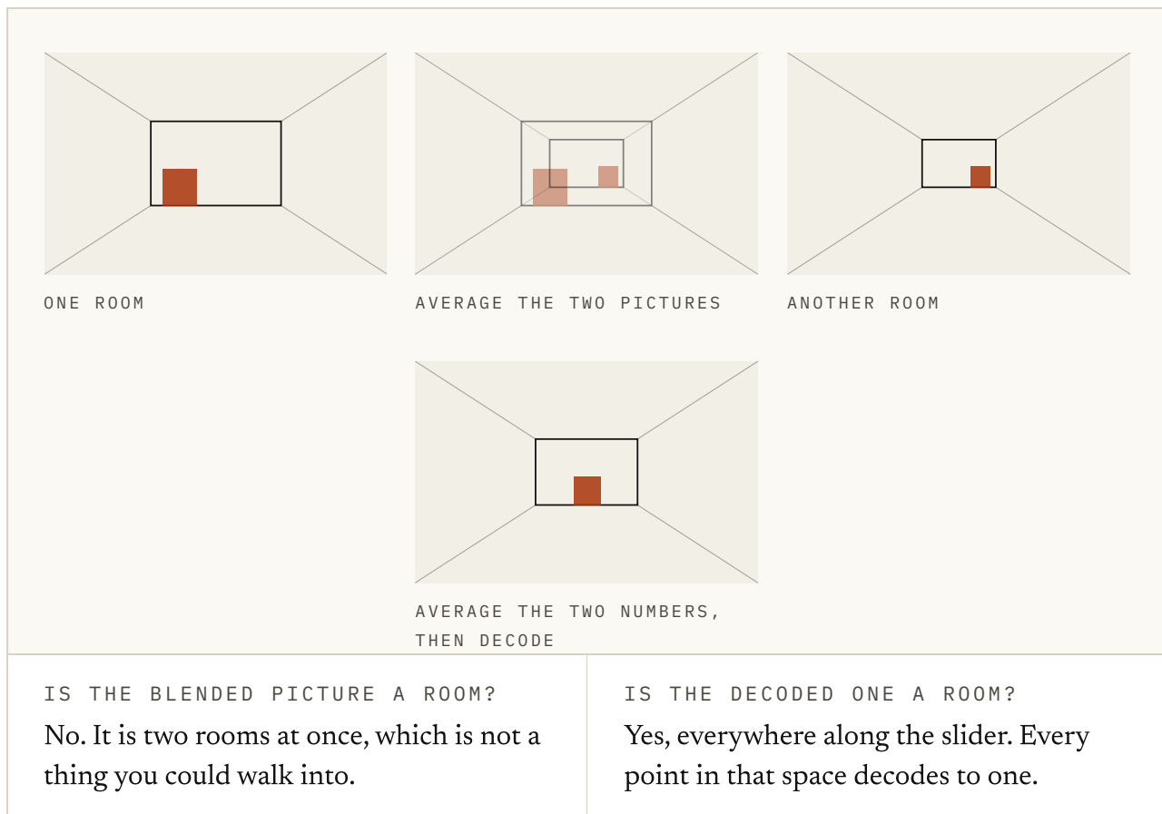
FIG. 4.3 Both rows are honest for this constructed decoder. Averaging two pictures gives you both rooms at once, faintly. Averaging the two coordinates and decoding stays on the learned room manifold. A real latent space only earns this behaviour if training has made the region between examples meaningful.
