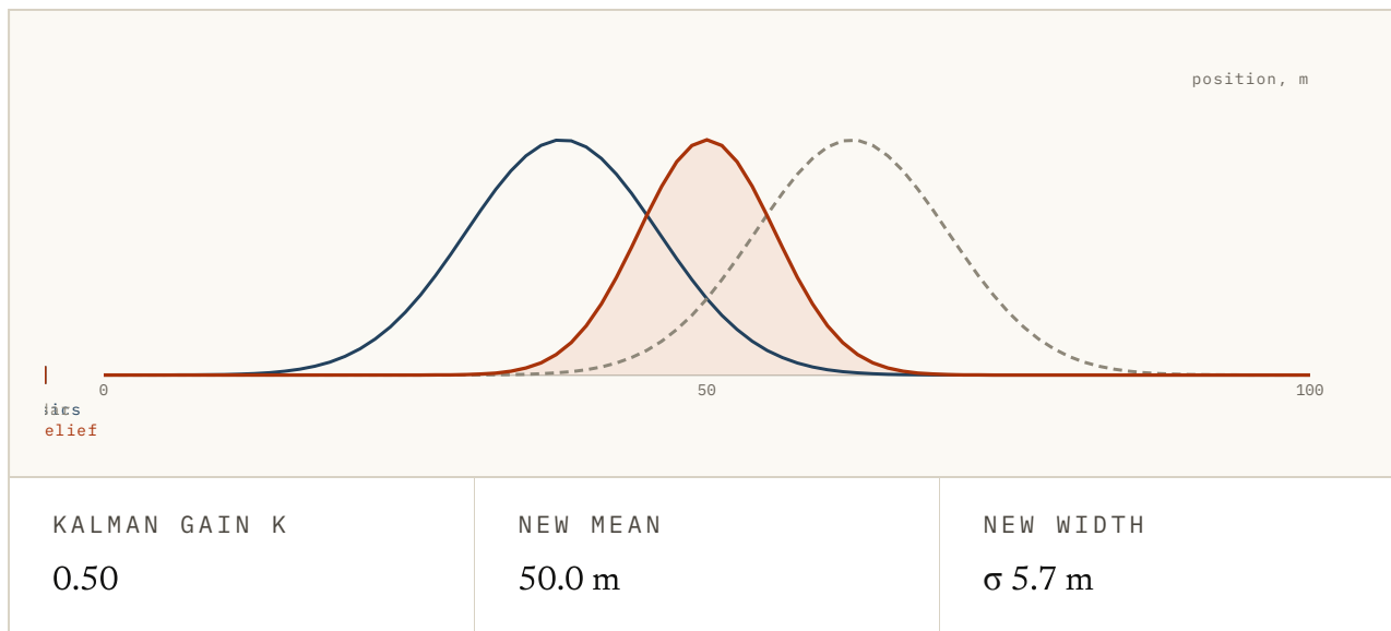
FIG. 5.3 Here are the two stories about where the plane is, drawn as bell curves on one axis. Slide how sure physics is and how noisy the radar is, and watch the new belief lean toward the sharper story while staying narrower than either. The gain is the number that says how far it leaned. Now press Correct to make the new belief the next physics prediction, and watch it widen again as the plane moves on.
