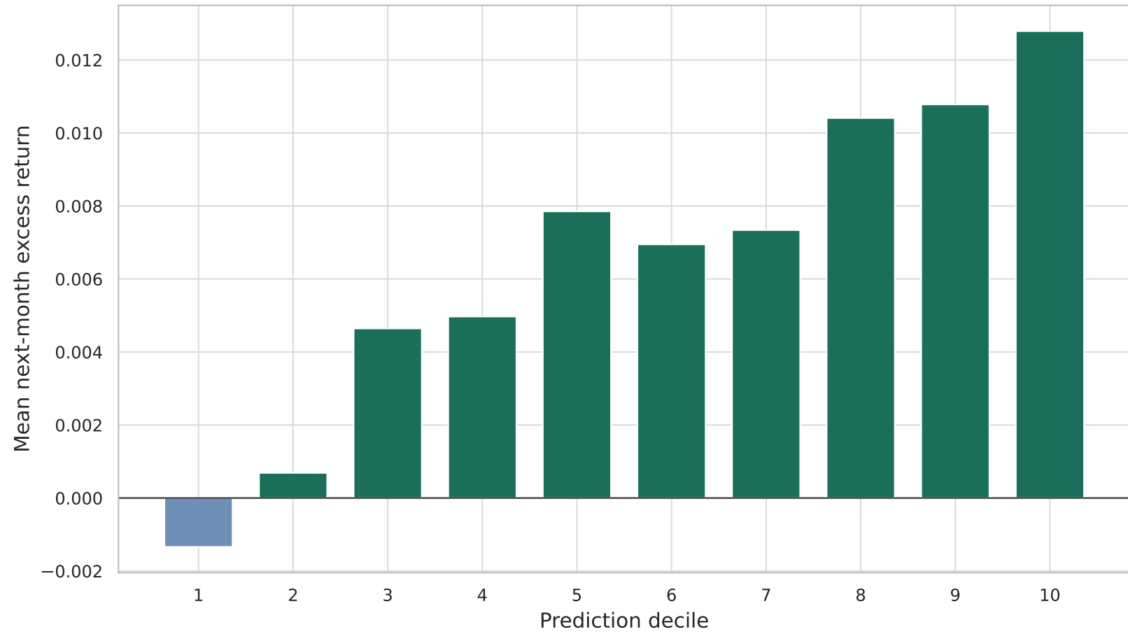
Realized Return by Prediction Decile (lightgbm)
