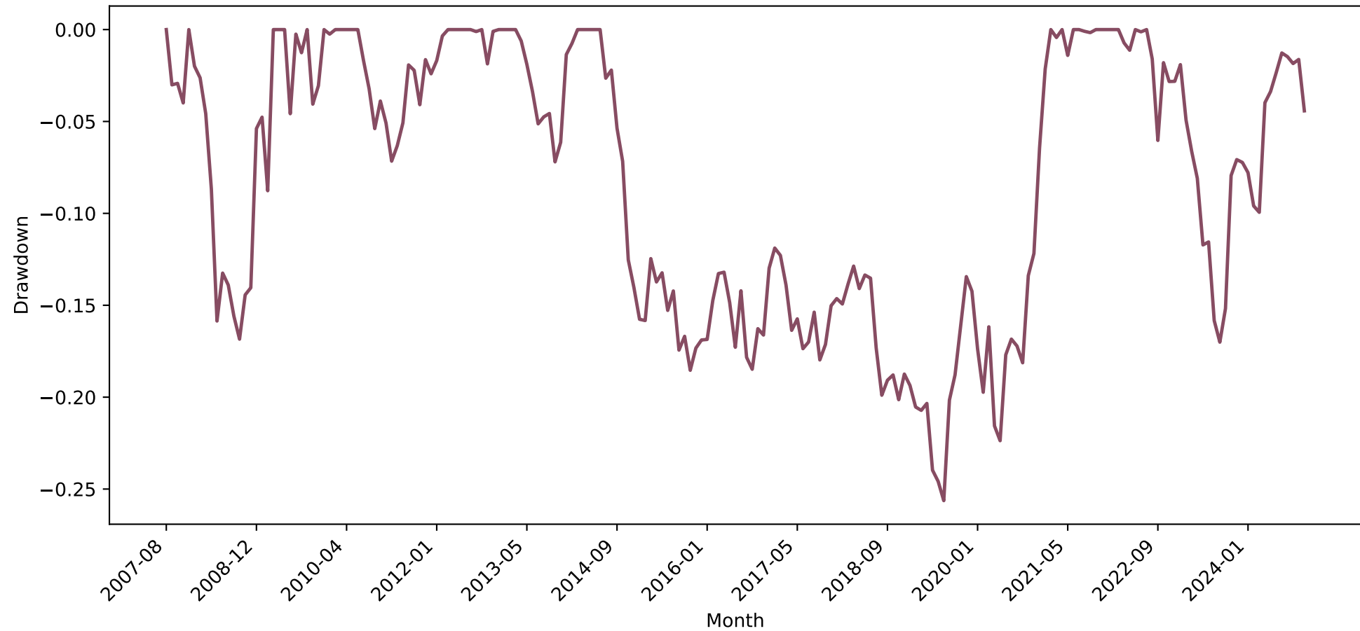
Long-Short Drawdown
