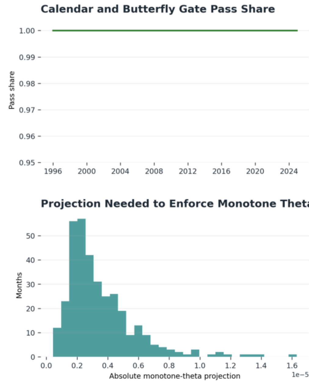
Figure 2. SSVI Surface Quality and No-Arbitrage Diagnostics
