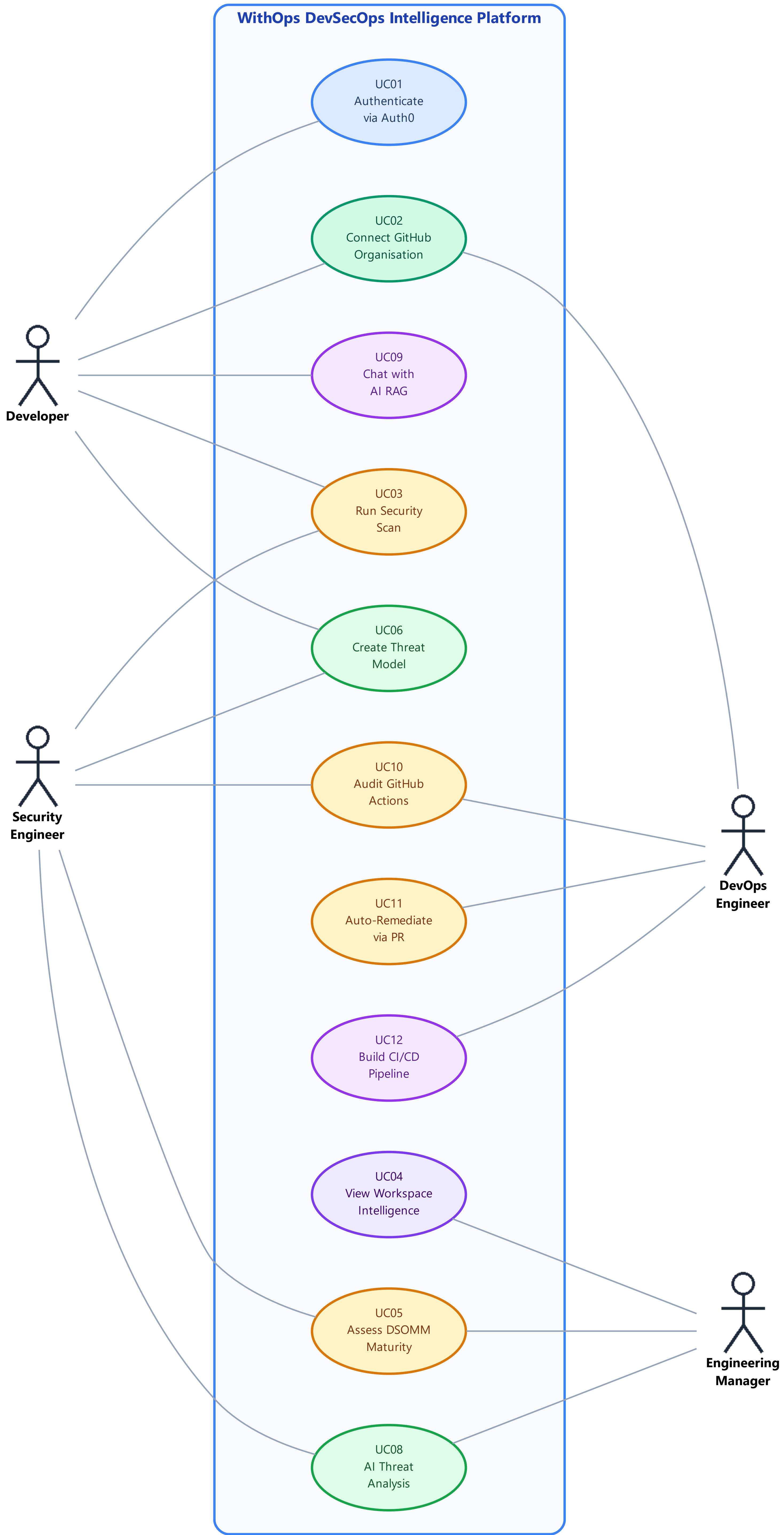
Figure 5.1 — WithOps Use Case Diagram
