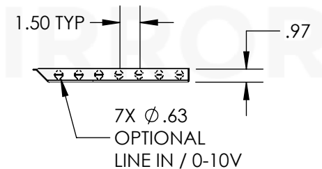
DETAIL A POWER BOX 81330-D1-DF-96W
