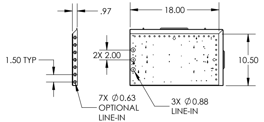
DETAIL A POWER BOX
