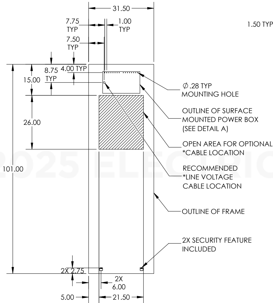
WALL MOUNTING DETAILS
