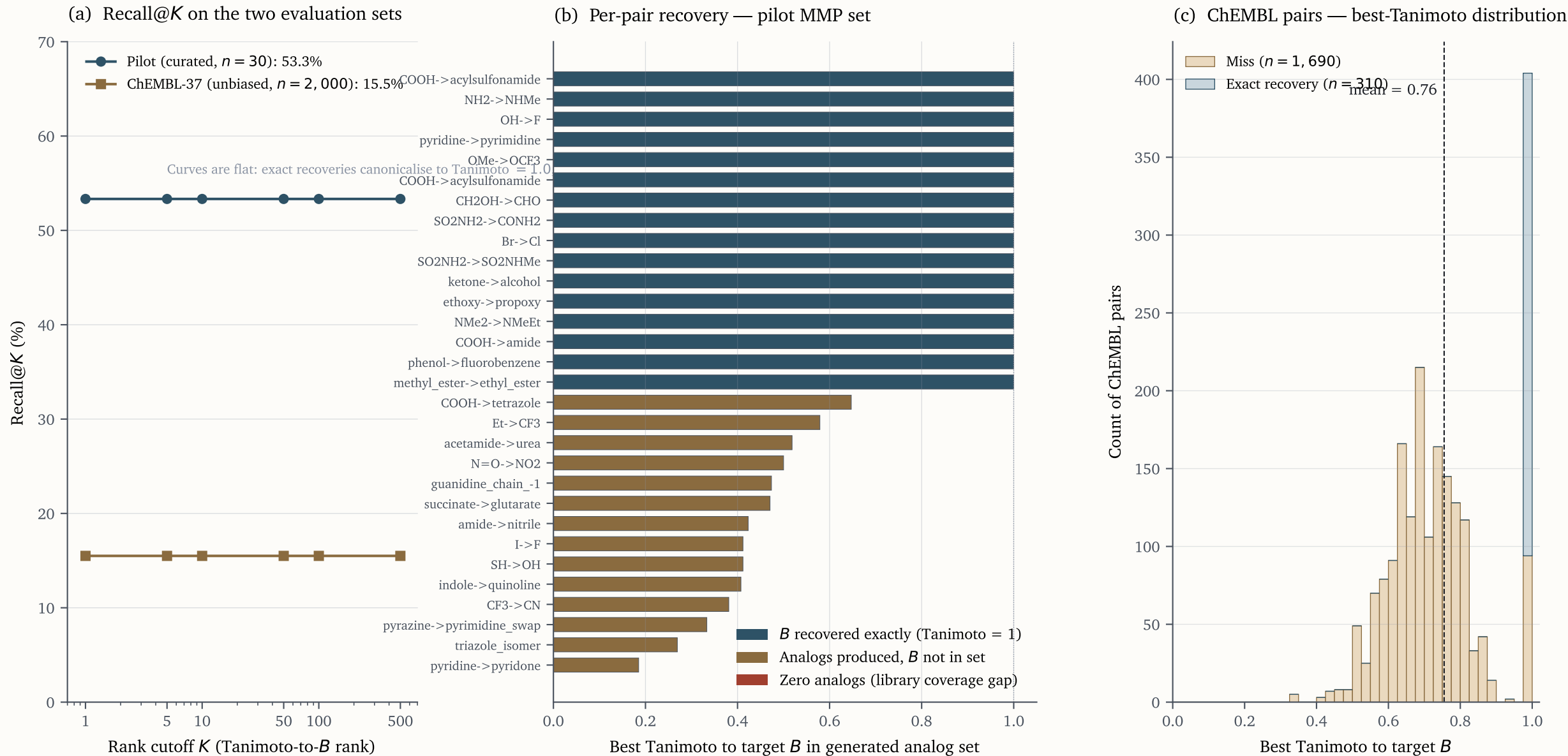
Figure 2 — MMP recovery on curated and unbiased evaluation sets Pilot: 30 literature-documented single-edit pairs (upper bound on the library's native domain). ChEMBL-37 scale-up: 2,000 unbiased single-edit pairs from a 2000-compound drug-like subset, built via mmpdb fragment + index. Library = 479 SMIRKS / 22 categories.
