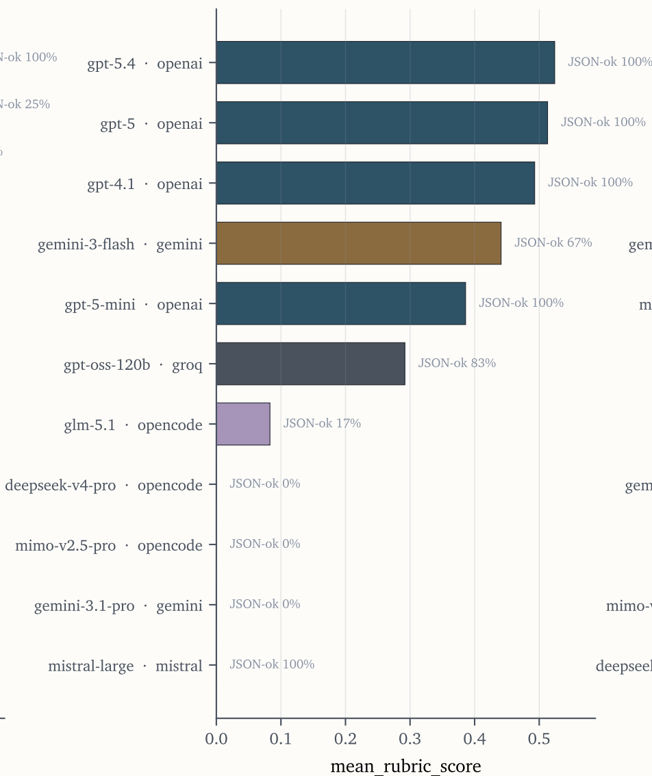
(b) Stage 5 — Project context · endpoint-priority rubric
