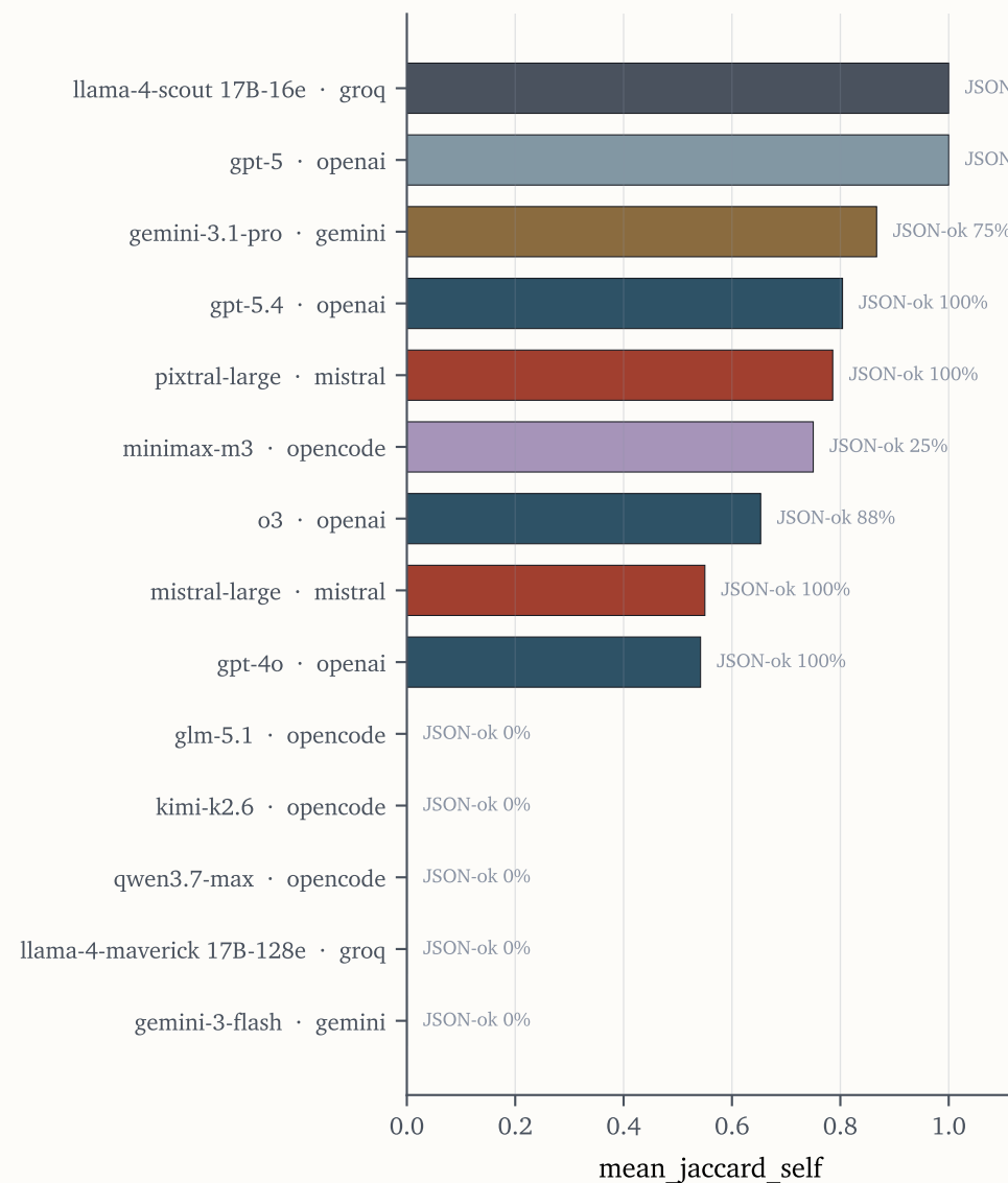
(a) Stage 2 — Vision Agent · self-consistency Jaccard
