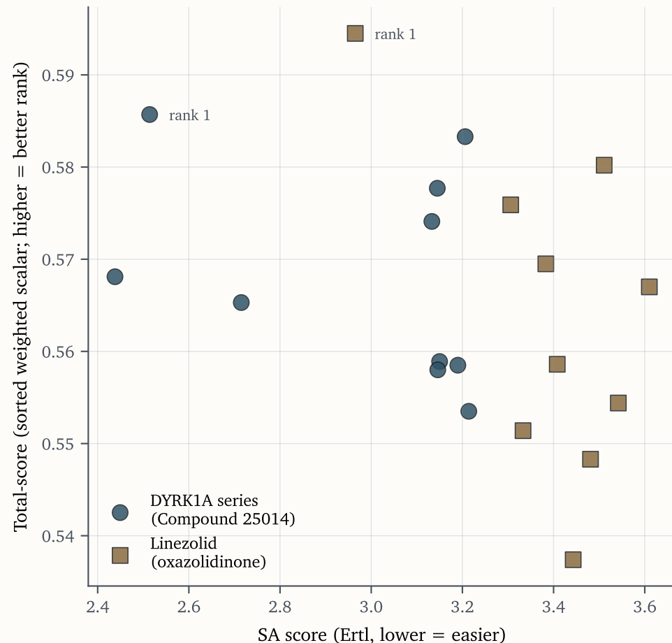
(b) Top-10 per case, total-score vs synthetic accessibility
