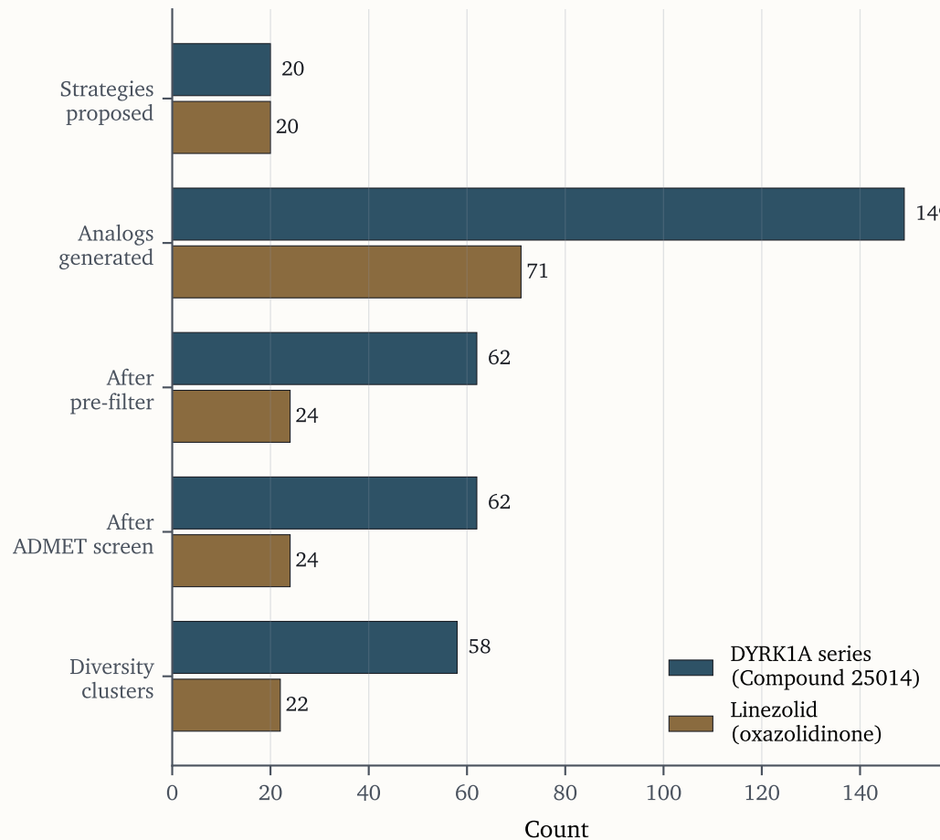
(a) Stage-by-stage attrition through the 12-stage pipeline
