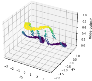
NLS dataset (nonlinearly separable, 3 classes) - FCNN 2-64-16-3 Hidden layer 2 node 5 - train data
