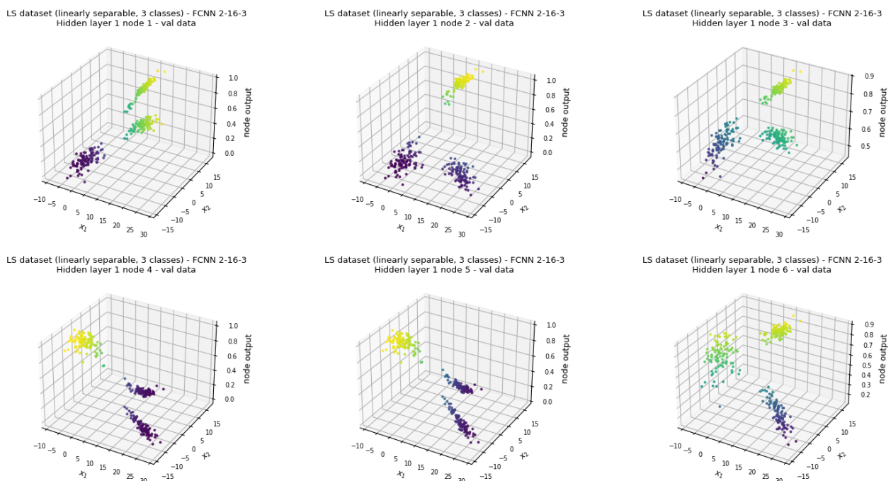
Figure 2.61v: outputs of hidden layer 1 nodes 1-6 of 16 (val data). Each node has its own figure; all 16 are in outputs/classification_ls/best_architecture/node_outputs/hidden_layer1/val/ .
