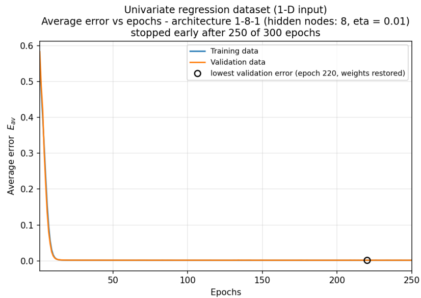
Figure 4.2a: average error vs epochs, architecture 1-8-1 (hidden nodes: 8).
