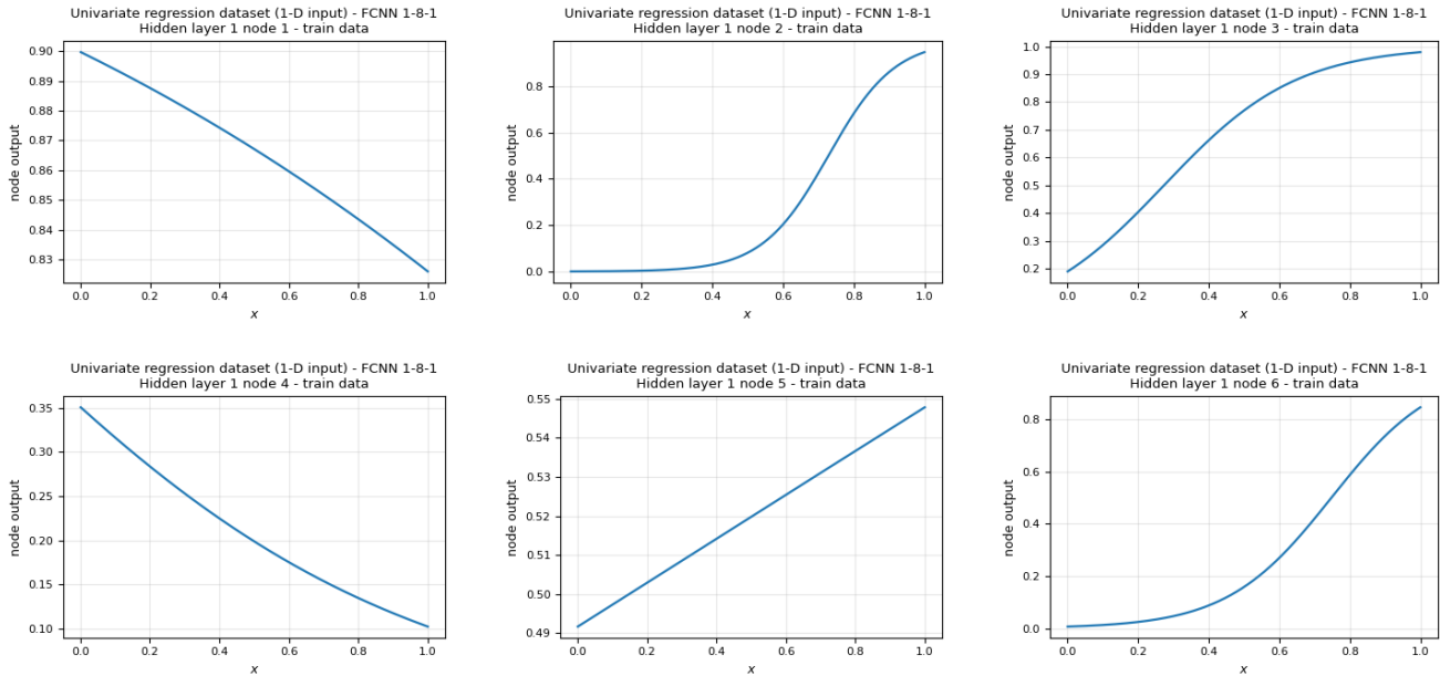
Figure 4.61t: outputs of hidden layer 1 nodes 1-6 of 8 (train data). Each node has its own figure; all 8 are in outputs/regression_univariate/best_architecture/node_outputs/hidden_layer1/train/ .
