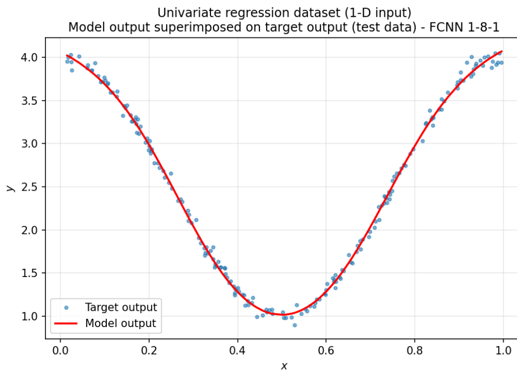
Figure 4.4t: model output superimposed on the target output (test data).
