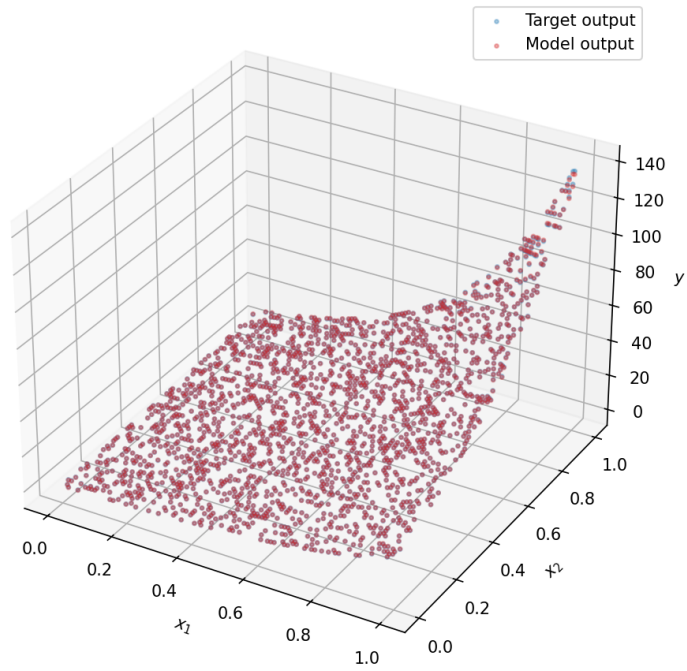
Figure 5.4t: model output superimposed on the target output (test data).
