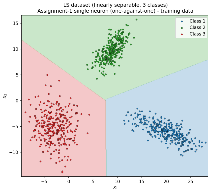
Figure 2.5: decision regions of the Assignment-1 single-neuron model on the same training data.
