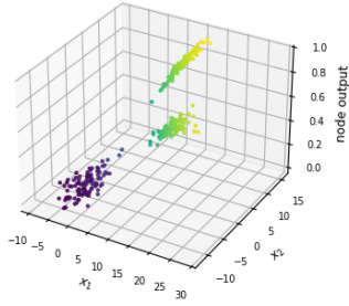
LS dataset (linearly separable, 3 classes) - FCNN 2-16-3 Hidden layer 1 node 4 - test data
