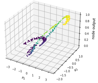
Figure 3.61t: outputs of hidden layer 1 nodes 1-6 of 64 (test data). Each node has its own figure; all 64 are in outputs/classification_nls/best_architecture/node_outputs/hidden_layer1/test/ .
