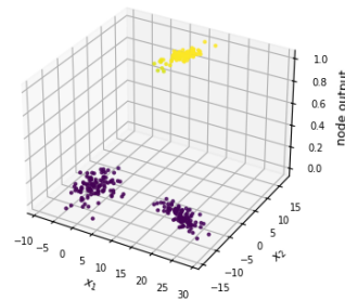
Figure 2.7v: outputs of all 3 output nodes (val data), one figure per node.
