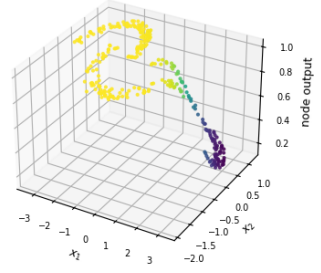
NLS dataset (nonlinearly separable, 3 classes) - FCNN 2-64-16-3 Hidden layer 2 node 6 - test data
