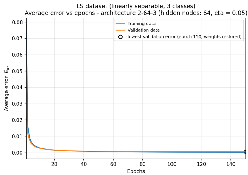
Figure 2.2d: average error vs epochs, architecture 2-64-3 (hidden nodes: 64).
