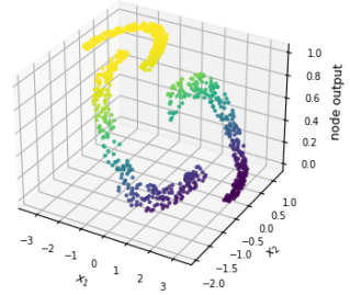
NLS dataset (nonlinearly separable, 3 classes) - FCNN 2-64-16-3 Hidden layer 1 node 6 - train data
