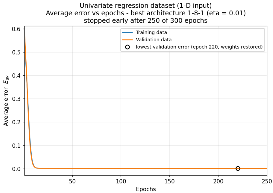
Figure 4.3: average error E_{av} against epochs for the best architecture.
