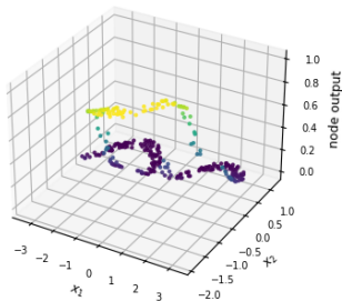
NLS dataset (nonlinearly separable, 3 classes) - FCNN 2-64-16-3 Hidden layer 2 node 4 - val data
