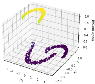
Figure 3.7t: outputs of all 3 output nodes (train data), one figure per node.
