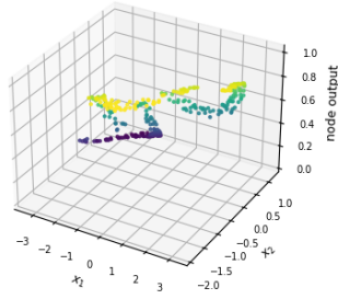
NLS dataset (nonlinearly separable, 3 classes) - FCNN 2-64-16-3 Hidden layer 1 node 5 - test data
