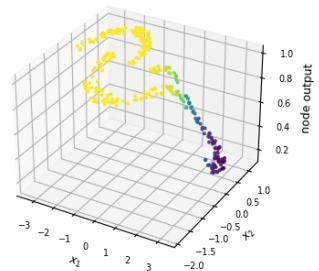
NLS dataset (nonlinearly separable, 3 classes) - FCNN 2-64-16-3 Hidden layer 2 node 6 - val data
