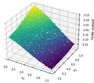
Bivariate regression dataset (2-D input) - FCNN 2-64-32-1 Hidden layer 2 node 5 - train data
