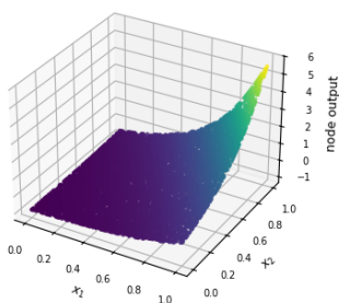
Figure 5.7t: outputs of all 1 output node (train data), one figure per node.
