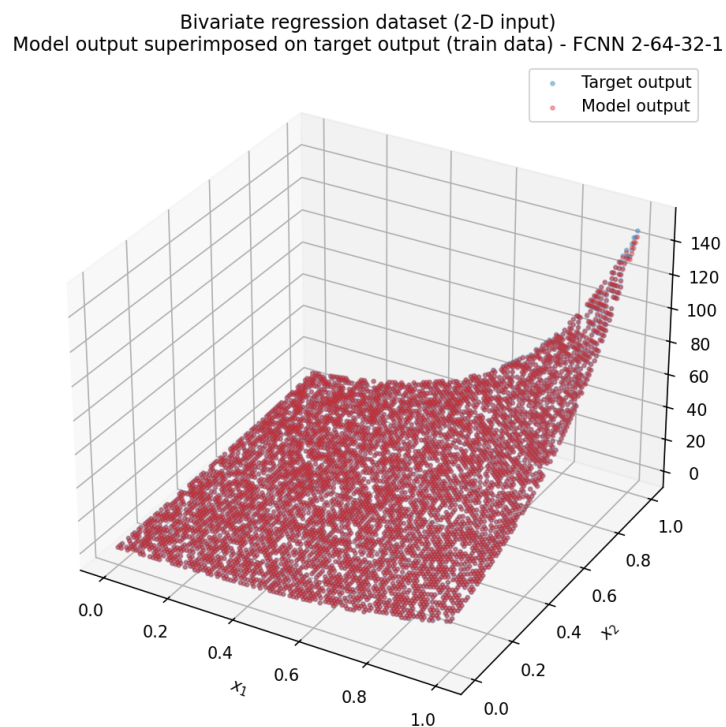
Figure 5.4t: model output superimposed on the target output (train data).
