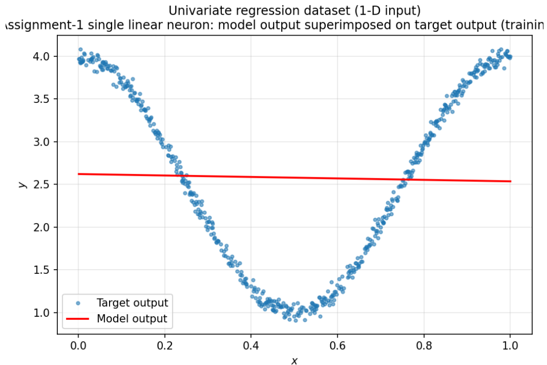
Figure 4.6: the Assignment-1 single linear neuron on the same training data.
