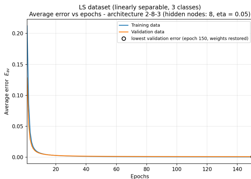
Figure 2.2a: average error vs epochs, architecture 2-8-3 (hidden nodes: 8).
