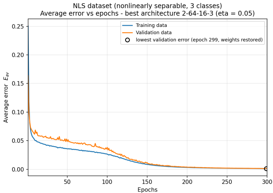
Figure 3.3: average error E_{av} against epochs for the best architecture.
