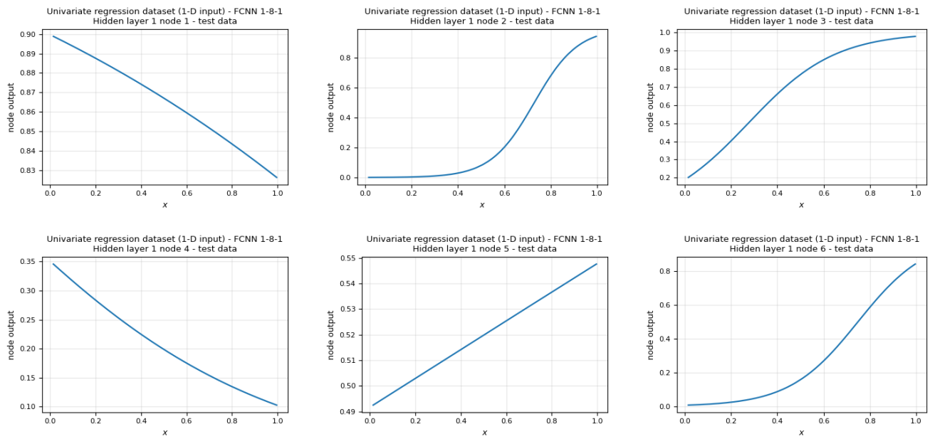
Figure 4.61t: outputs of hidden layer 1 nodes 1-6 of 8 (test data). Each node has its own figure; all 8 are in outputs/regression_univariate/best_architecture/node_outputs/hidden_layer1/test/ .
