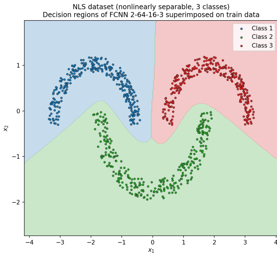
Figure 3.4: decision regions of the best FCNN, superimposed on the training data.
