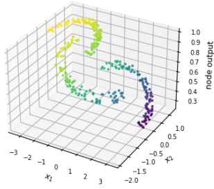
NLS dataset (nonlinearly separable, 3 classes) - FCNN 2-64-16-3 Hidden layer 1 node 4 - test data
