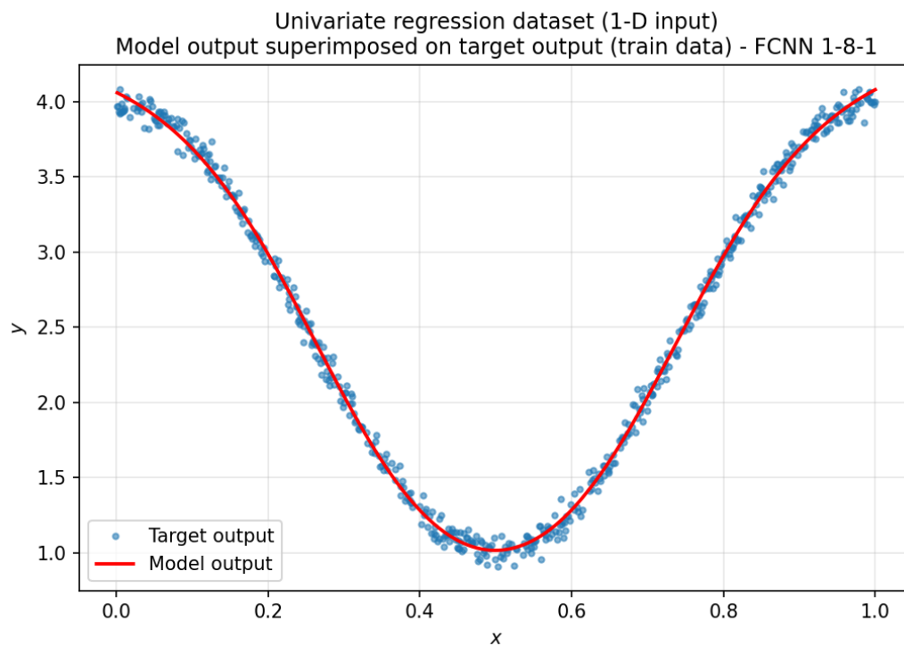
Figure 4.4t: model output superimposed on the target output (train data).
