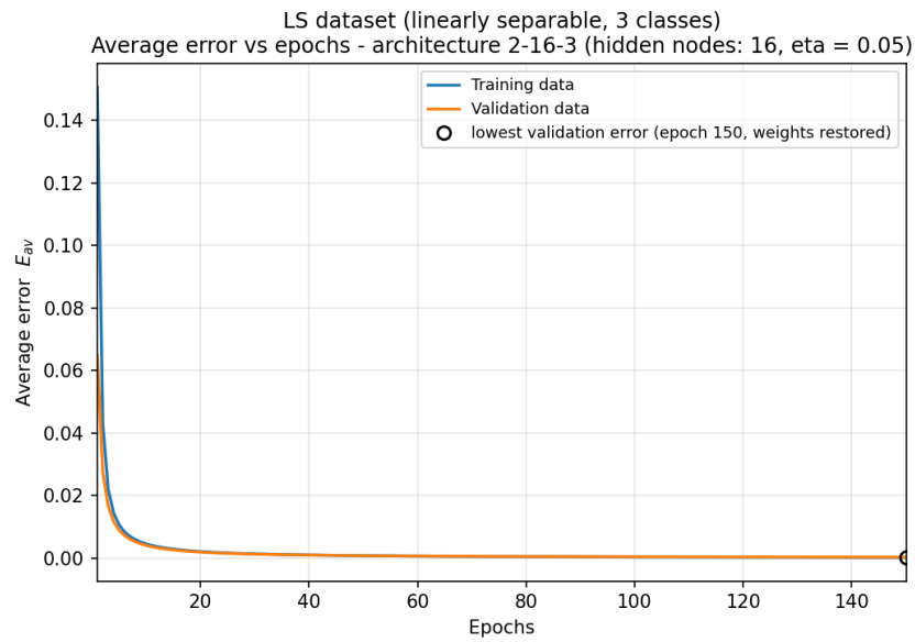
Figure 2.2b: average error vs epochs, architecture 2-16-3 (hidden nodes: 16).
