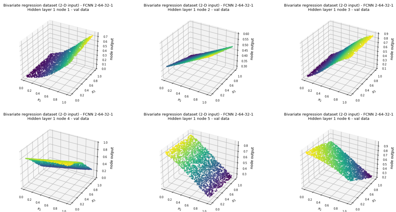
Figure 5.61v: outputs of hidden layer 1 nodes 1-6 of 64 (val data). Each node has its own figure; all 64 are in outputs/regression_bivariate/best_architecture/node_outputs/hidden_layer1/val/ .
