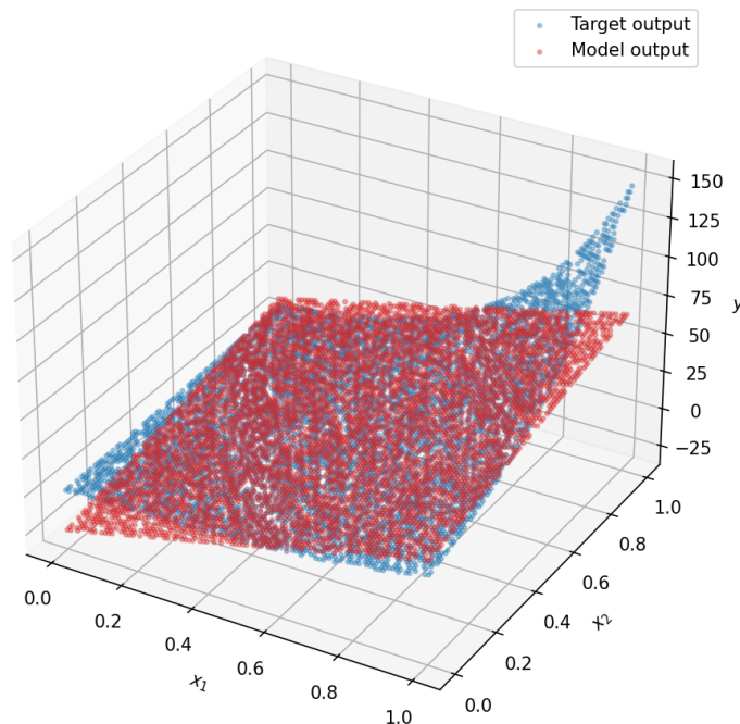
Figure 5.6: the Assignment-1 single linear neuron on the same training data.
