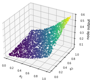
Bivariate regression dataset (2-D input) - FCNN 2-64-32-1 Hidden layer 2 node 4 - val data
