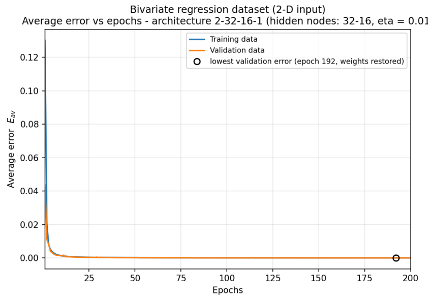
Figure 5.2d: average error vs epochs, architecture 2-32-16-1 (hidden nodes: 32-16).
