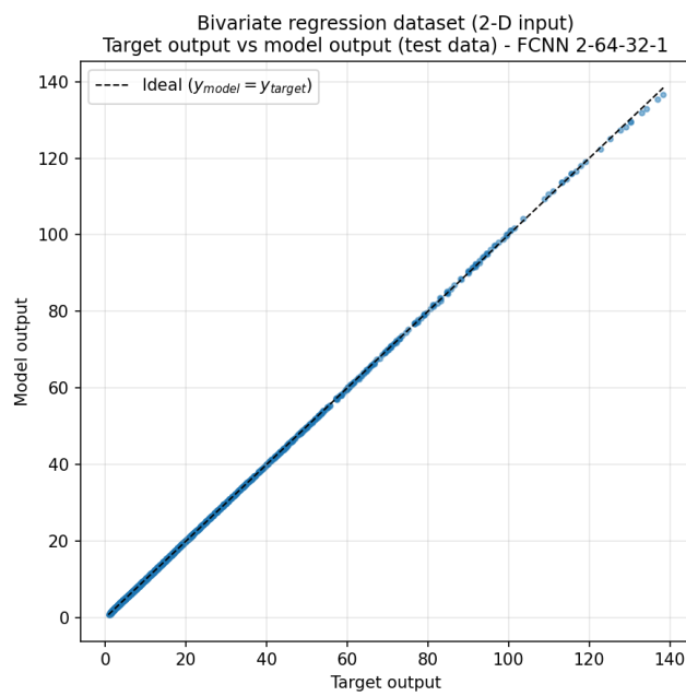
Figure 5.5t: target output (x-axis) vs model output (y-axis), test data.
