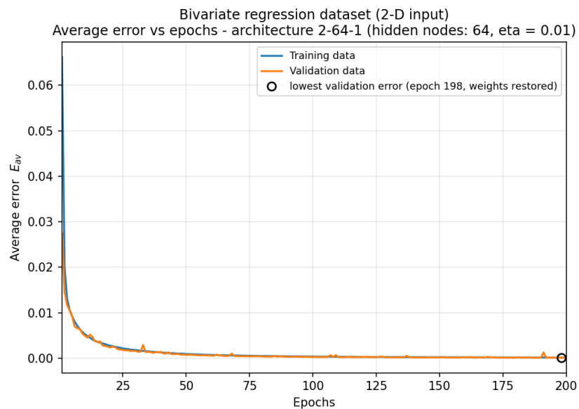
Figure 5.2c: average error vs epochs, architecture 2-64-1 (hidden nodes: 64).
