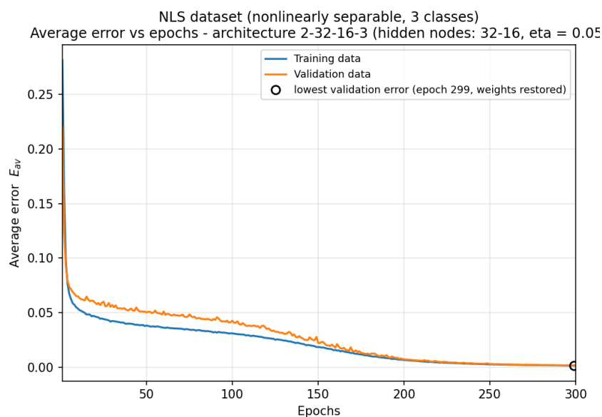
Figure 3.2b: average error vs epochs, architecture 2-32-16-3 (hidden nodes: 32-16).
