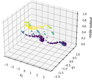
NLS dataset (nonlinearly separable, 3 classes) - FCNN 2-64-16-3 Hidden layer 2 node 5 - test data
