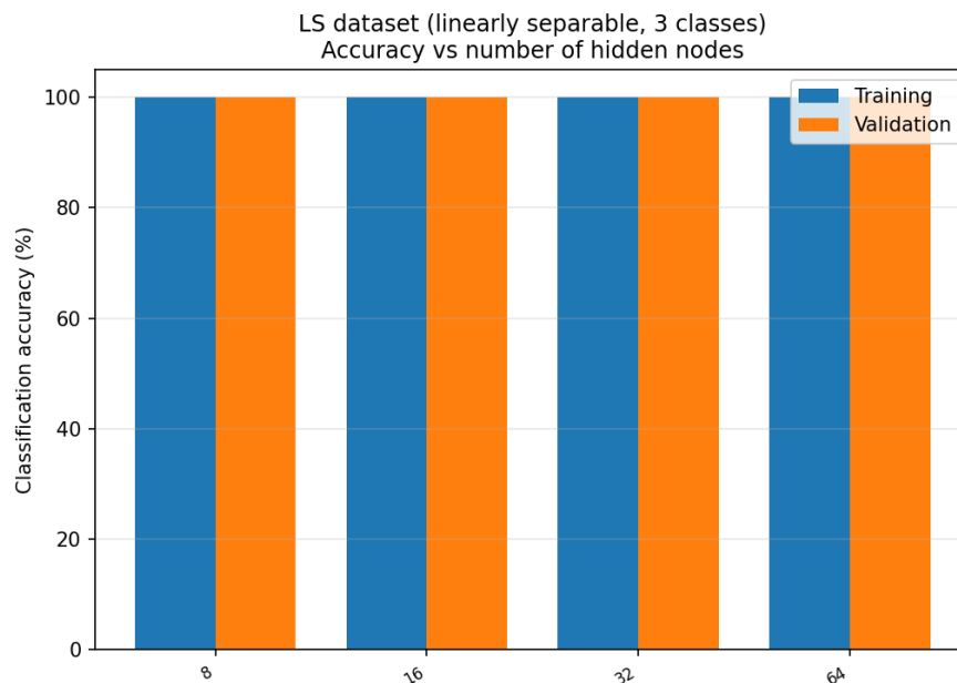
Figure 2.1: training and validation accuracy against the number of hidden nodes.
