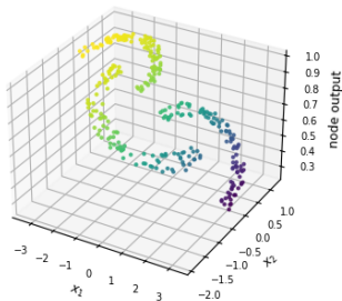
NLS dataset (nonlinearly separable, 3 classes) - FCNN 2-64-16-3 Hidden layer 1 node 4 - val data
