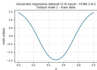
Figure 4.7t: outputs of all 1 output node (train data), one figure per node.
