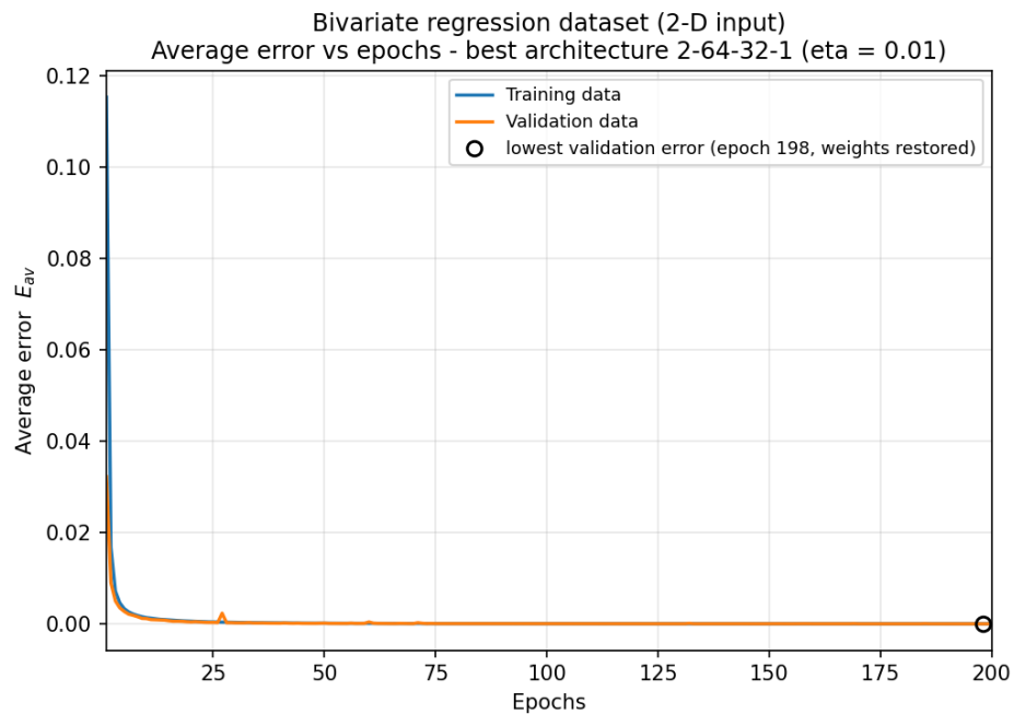
Figure 5.3: average error E_{av} against epochs for the best architecture.
