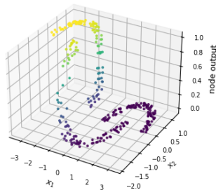
Figure 3.62v: outputs of hidden layer 2 nodes 1-6 of 16 (val data). Each node has its own figure; all 16 are in outputs/classification_nls/best_architecture/node_outputs/hidden_layer2/val/ .
