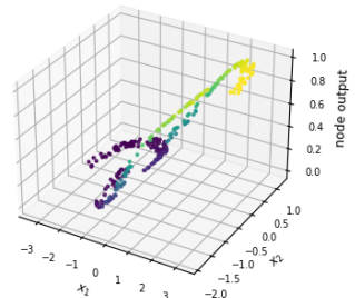
Figure 3.61v: outputs of hidden layer 1 nodes 1-6 of 64 (val data). Each node has its own figure; all 64 are in outputs/classification_nls/best_architecture/node_outputs/hidden_layer1/val/ .
