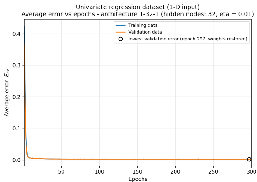
Figure 4.2c: average error vs epochs, architecture 1-32-1 (hidden nodes: 32).
