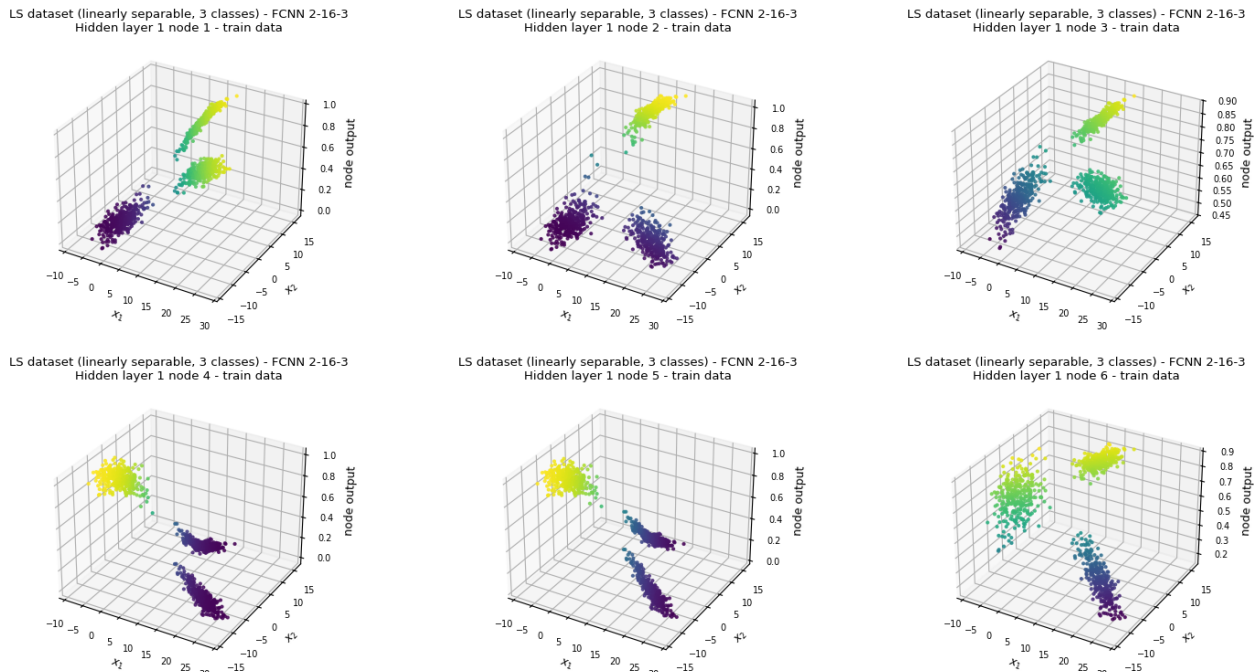
Figure 2.61t: outputs of hidden layer 1 nodes 1-6 of 16 (train data). Each node has its own figure; all 16 are in outputs/classification_ls/best_architecture/node_outputs/hidden_layer1/train/ .
