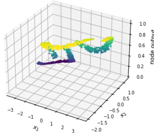
NLS dataset (nonlinearly separable, 3 classes) - FCNN 2-64-16-3 Hidden layer 1 node 5 - train data
