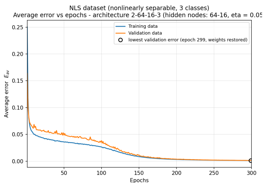
Figure 3.2c: average error vs epochs, architecture 2-64-16-3 (hidden nodes: 64-16).
