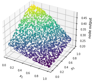
Figure 5.62t: outputs of hidden layer 2 nodes 1-6 of 32 (test data). Each node has its own figure; all 32 are in outputs/regression_bivariate/best_architecture/node_outputs/hidden_layer2/test/ .
