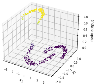
Figure 3.7v: outputs of all 3 output nodes (val data), one figure per node.
