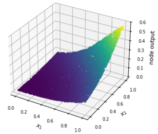
Bivariate regression dataset (2-D input) - FCNN 2-64-32-1 Hidden layer 2 node 6 - train data
