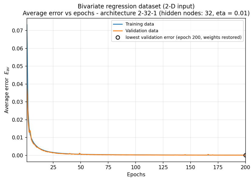
Figure 5.2b: average error vs epochs, architecture 2-32-1 (hidden nodes: 32).
