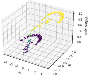
Figure 3.62t: outputs of hidden layer 2 nodes 1-6 of 16 (test data). Each node has its own figure; all 16 are in outputs/classification_nls/best_architecture/node_outputs/hidden_layer2/test/ .
