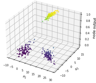
LS dataset (linearly separable, 3 classes) - FCNN 2-16-3 Hidden layer 1 node 5 - test data
