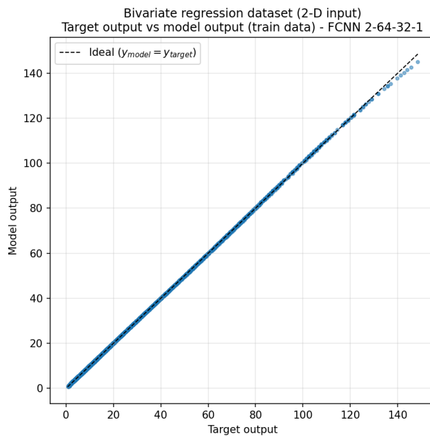
Figure 5.5t: target output (x-axis) vs model output (y-axis), train data.
