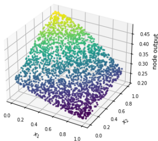
Figure 5.62v: outputs of hidden layer 2 nodes 1-6 of 32 (val data). Each node has its own figure; all 32 are in outputs/regression_bivariate/best_architecture/node_outputs/hidden_layer2/val/ .
