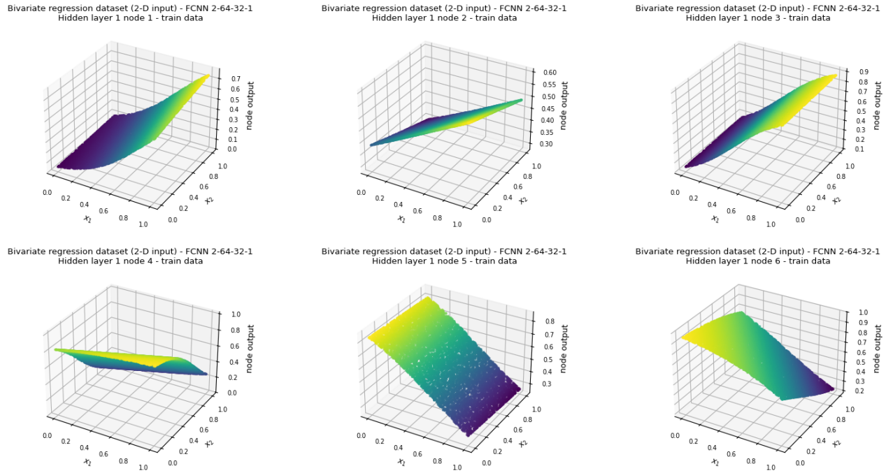
Figure 5.61t: outputs of hidden layer 1 nodes 1-6 of 64 (train data). Each node has its own figure; all 64 are in outputs/regression_bivariate/best_architecture/node_outputs/hidden_layer1/train/ .
