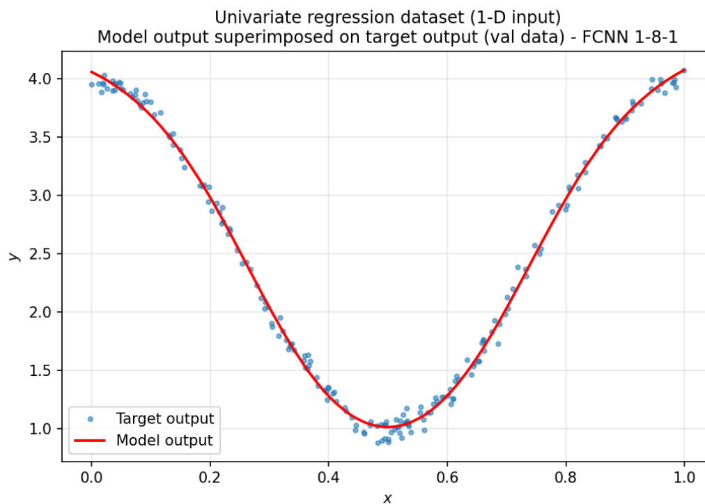
Figure 4.4v: model output superimposed on the target output (val data).
