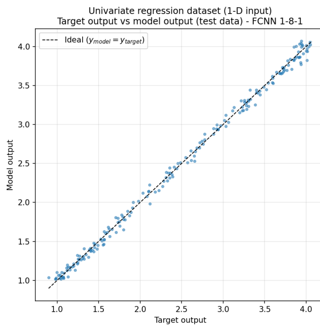
Figure 4.5t: target output (x-axis) vs model output (y-axis), test data.
