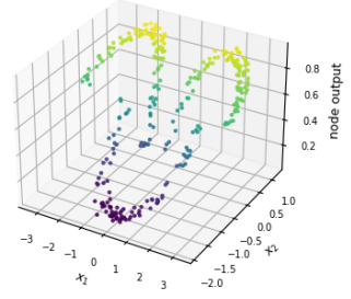
Figure 3.62t: outputs of hidden layer 2 nodes 1-6 of 16 (test data). Each node has its own figure; all 16 are in outputs/classification_nls/best_architecture/node_outputs/hidden_layer2/test/ .
