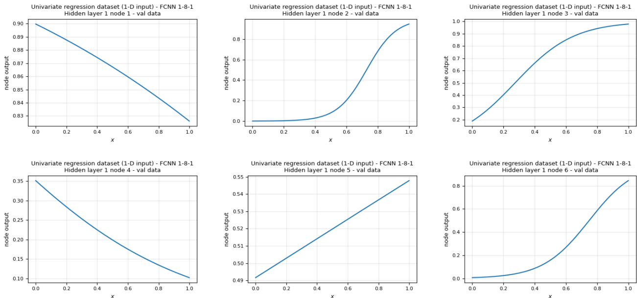
Figure 4.61v: outputs of hidden layer 1 nodes 1-6 of 8 (val data). Each node has its own figure; all 8 are in outputs/regression_univariate/best_architecture/node_outputs/hidden_layer1/val/ .
