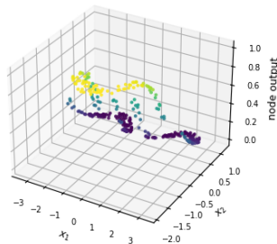
NLS dataset (nonlinearly separable, 3 classes) - FCNN 2-64-16-3 Hidden layer 2 node 5 - val data
