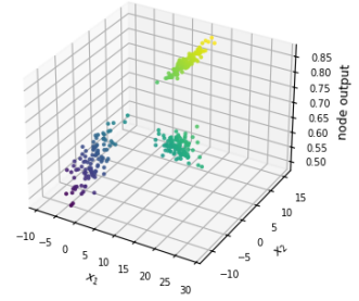
LS dataset (linearly separable, 3 classes) - FCNN 2-16-3 Hidden layer 1 node 6 - test data
