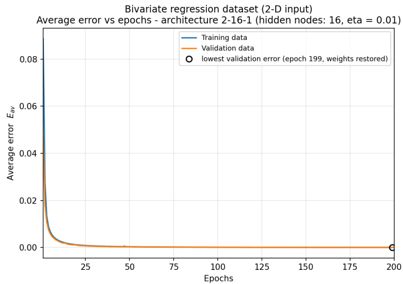
Figure 5.2a: average error vs epochs, architecture 2-16-1 (hidden nodes: 16).
