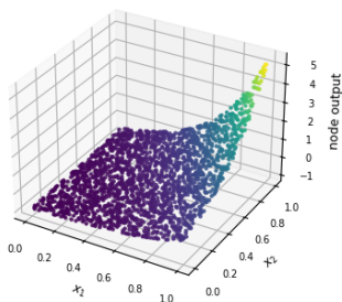
Figure 5.7t: outputs of all 1 output node (test data), one figure per node.
