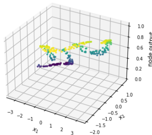
NLS dataset (nonlinearly separable, 3 classes) - FCNN 2-64-16-3 Hidden layer 1 node 5 - val data
