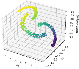
NLS dataset (nonlinearly separable, 3 classes) - FCNN 2-64-16-3 Hidden layer 1 node 4 - train data
