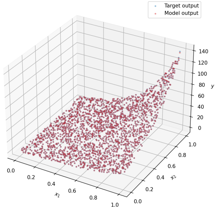
Figure 5.4v: model output superimposed on the target output (val data).
