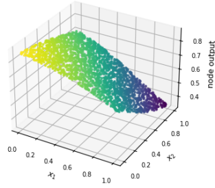
Figure 5.62t: outputs of hidden layer 2 nodes 1-6 of 32 (test data). Each node has its own figure; all 32 are in outputs/regression_bivariate/best_architecture/node_outputs/hidden_layer2/test/ .
