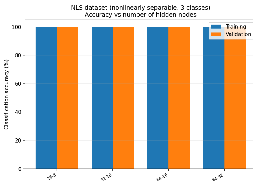
Figure 3.1: training and validation accuracy against the number of hidden nodes.
