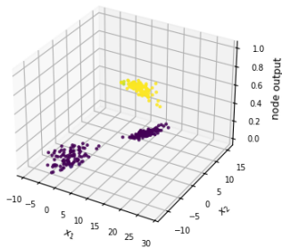
Figure 2.7t: outputs of all 3 output nodes (test data), one figure per node.
