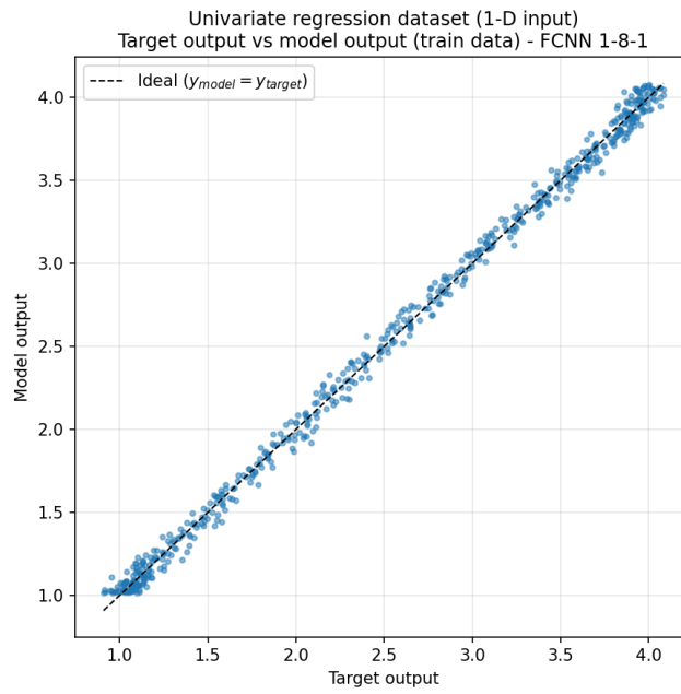
Figure 4.5t: target output (x-axis) vs model output (y-axis), train data.
