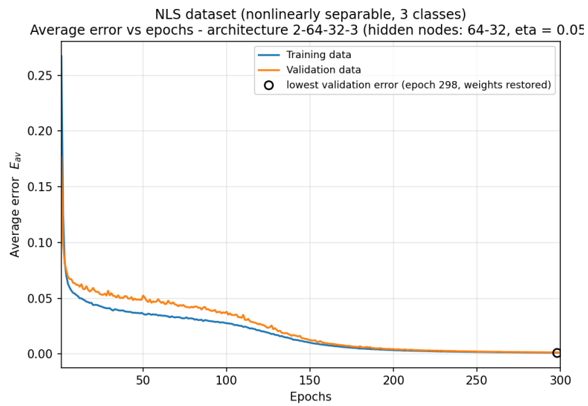
Figure 3.2d: average error vs epochs, architecture 2-64-32-3 (hidden nodes: 64-32).
