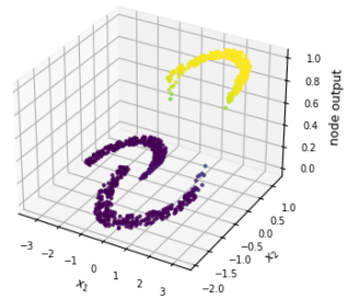
Figure 3.7t: outputs of all 3 output nodes (train data), one figure per node.
