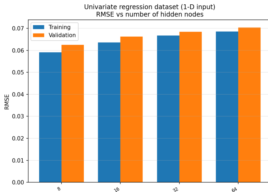
Figure 4.1: RMSE against the number of hidden nodes.
