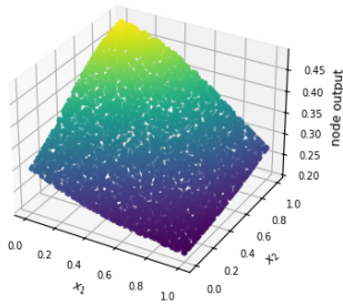
Figure 5.62t: outputs of hidden layer 2 nodes 1-6 of 32 (train data). Each node has its own figure; all 32 are in outputs/regression_bivariate/best_architecture/node_outputs/hidden_layer2/train/ .
