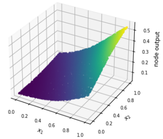
Figure 5.62t: outputs of hidden layer 2 nodes 1-6 of 32 (train data). Each node has its own figure; all 32 are in outputs/regression_bivariate/best_architecture/node_outputs/hidden_layer2/train/ .
