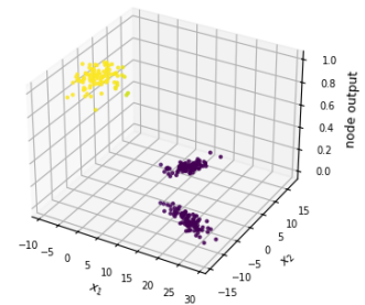
Figure 2.7v: outputs of all 3 output nodes (val data), one figure per node.
