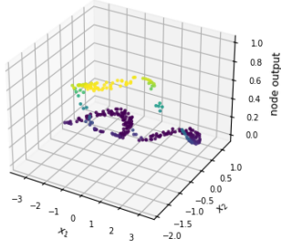
NLS dataset (nonlinearly separable, 3 classes) - FCNN 2-64-16-3 Hidden layer 2 node 4 - test data
