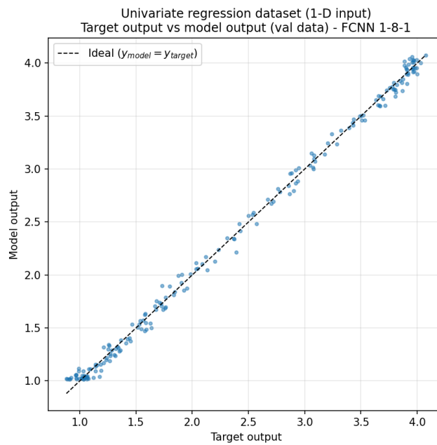
Figure 4.5v: target output (x-axis) vs model output (y-axis), val data.
