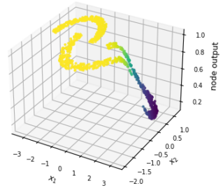
NLS dataset (nonlinearly separable, 3 classes) - FCNN 2-64-16-3 Hidden layer 2 node 6 - train data
