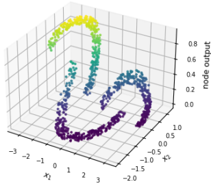
Figure 3.61t: outputs of hidden layer 1 nodes 1-6 of 64 (train data). Each node has its own figure; all 64 are in outputs/classification_nls/best_architecture/node_outputs/hidden_layer1/train/ .
