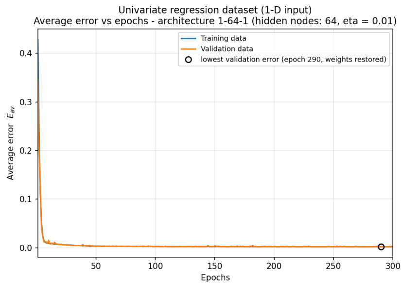
Figure 4.2d: average error vs epochs, architecture 1-64-1 (hidden nodes: 64).
