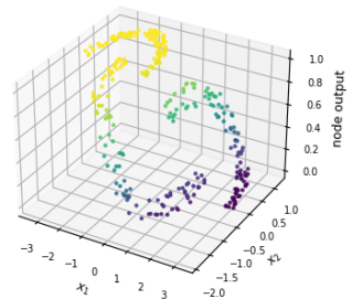
NLS dataset (nonlinearly separable, 3 classes) - FCNN 2-64-16-3 Hidden layer 1 node 6 - val data
