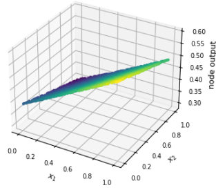
Bivariate regression dataset (2-D input) - FCNN 2-64-32-1 Hidden layer 1 node 5 - test data
