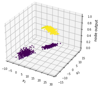
Figure 2.7t: outputs of all 3 output nodes (train data), one figure per node.
