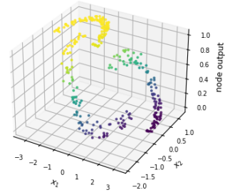
NLS dataset (nonlinearly separable, 3 classes) - FCNN 2-64-16-3 Hidden layer 1 node 6 - test data
