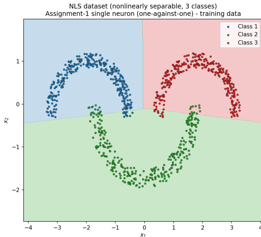
Figure 3.5: decision regions of the Assignment-1 single-neuron model on the same training data.
