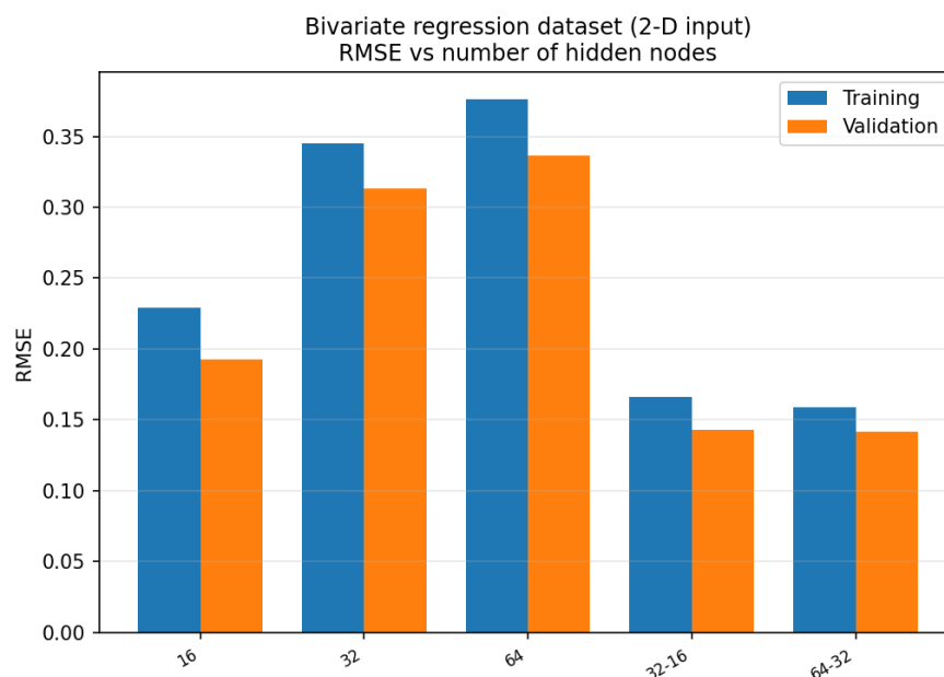
Figure 5.1: RMSE against the number of hidden nodes.
