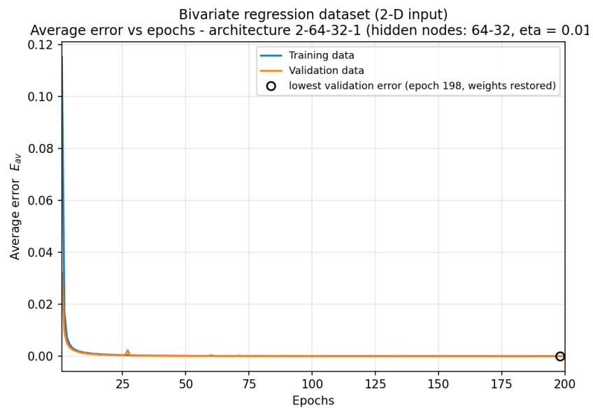
Figure 5.2e: average error vs epochs, architecture 2-64-32-1 (hidden nodes: 64-32).
