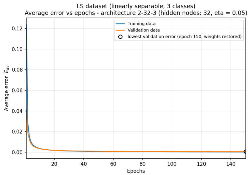
Figure 2.2c: average error vs epochs, architecture 2-32-3 (hidden nodes: 32).
