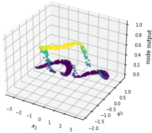
NLS dataset (nonlinearly separable, 3 classes) - FCNN 2-64-16-3 Hidden layer 2 node 4 - train data
