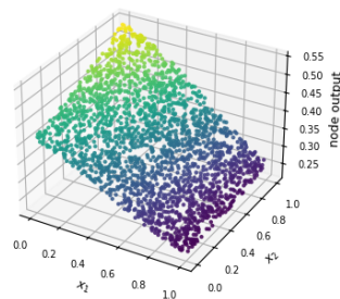
Bivariate regression dataset (2-D input) - FCNN 2-64-32-1 Hidden layer 2 node 5 - val data
