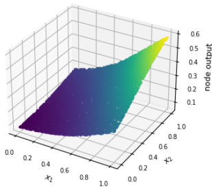
Bivariate regression dataset (2-D input) - FCNN 2-64-32-1 Hidden layer 2 node 4 - train data
