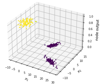
Figure 2.7t: outputs of all 3 output nodes (test data), one figure per node.
