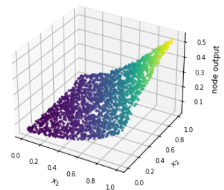
Figure 5.62v: outputs of hidden layer 2 nodes 1-6 of 32 (val data). Each node has its own figure; all 32 are in outputs/regression_bivariate/best_architecture/node_outputs/hidden_layer2/val/ .
