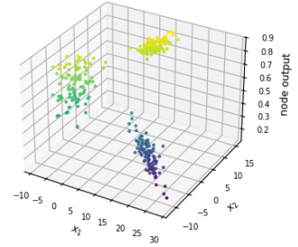
Figure 2.61t: outputs of hidden layer 1 nodes 1-6 of 16 (test data). Each node has its own figure; all 16 are in outputs/classification_ls/best_architecture/node_outputs/hidden_layer1/test/ .
