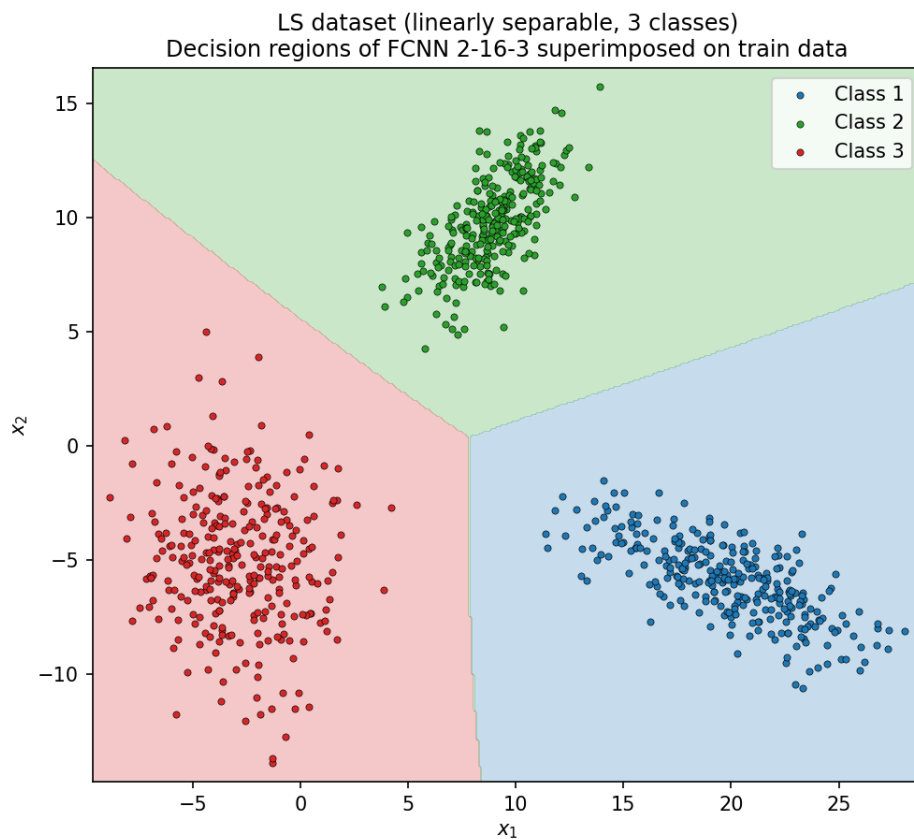
Figure 2.4: decision regions of the best FCNN, superimposed on the training data.
