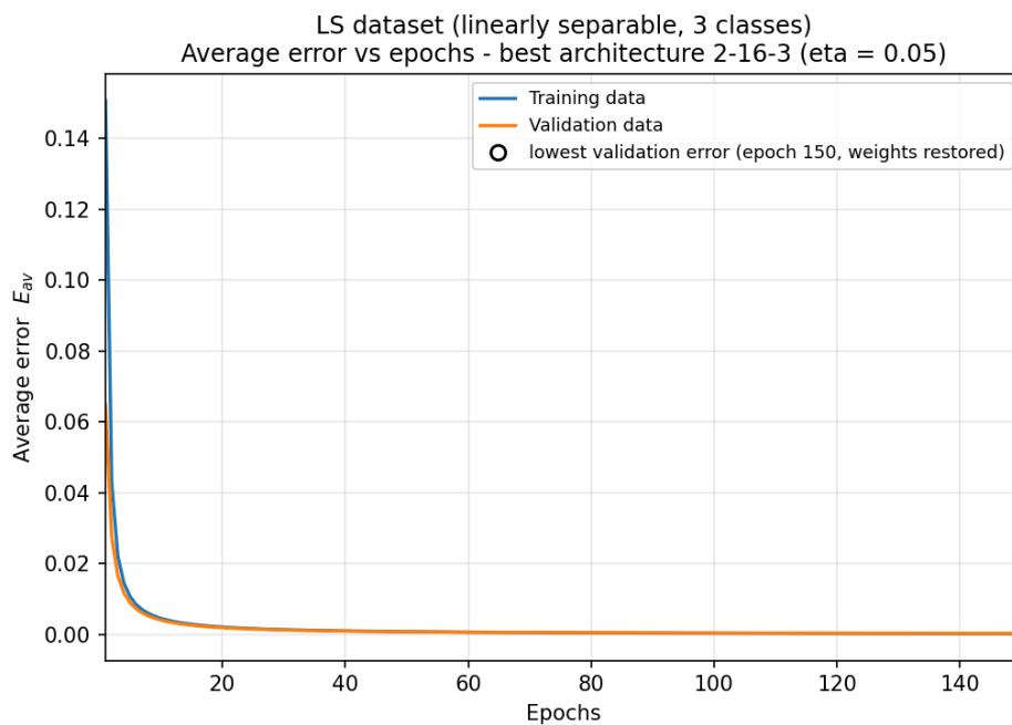
Figure 2.3: average error E_{av} against epochs for the best architecture.
