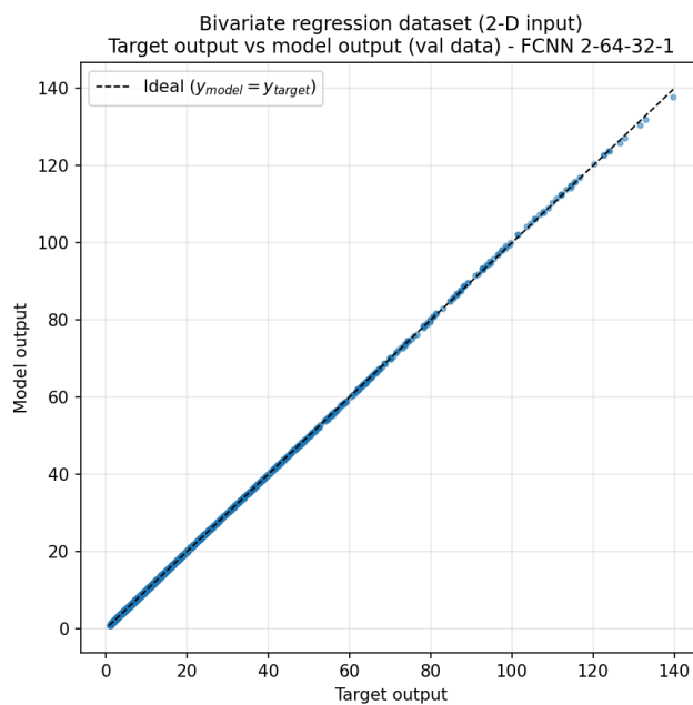
Figure 5.5v: target output (x-axis) vs model output (y-axis), val data.
