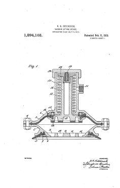
US-1294103-A · drawing
