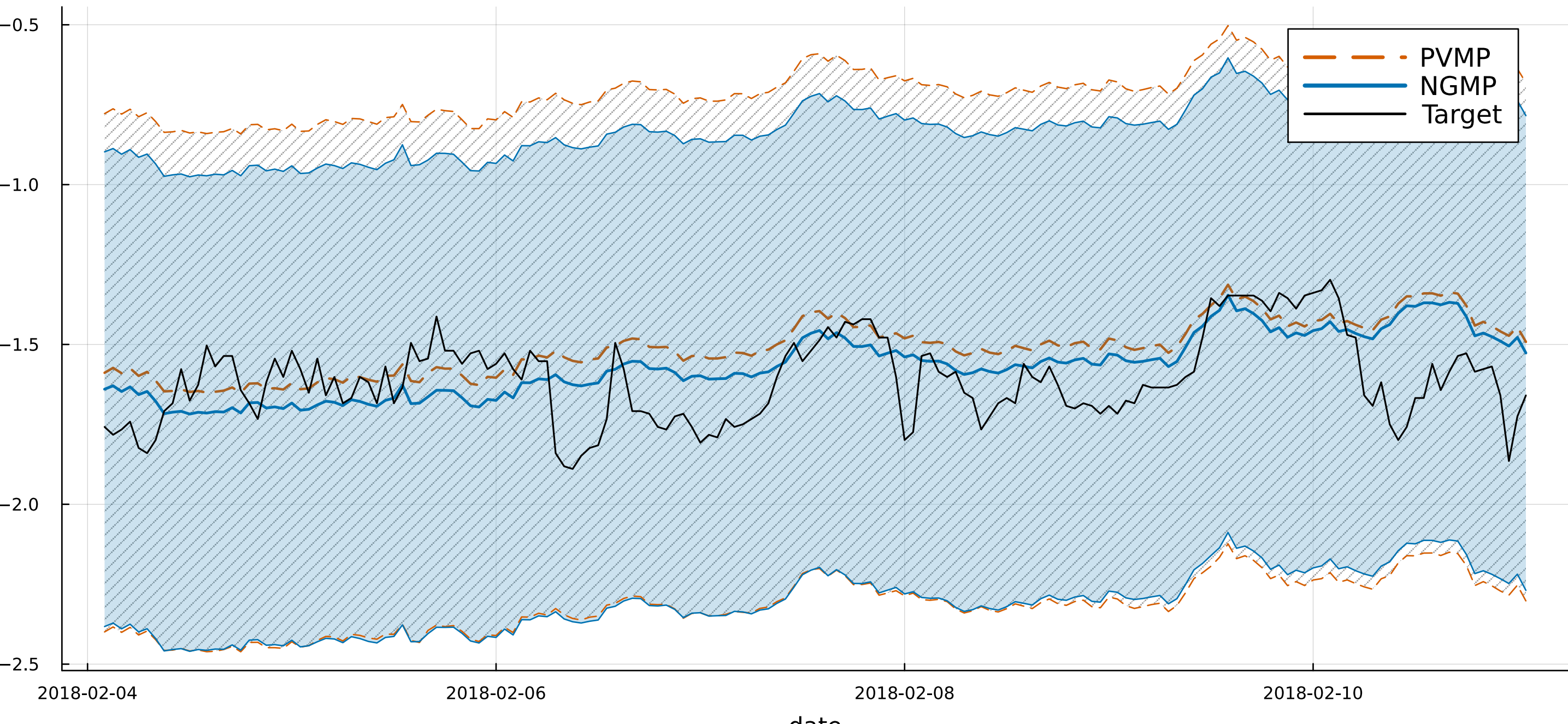
ETTh1, H=192: NGMP versus projective VMP (first 168 test predictions)
