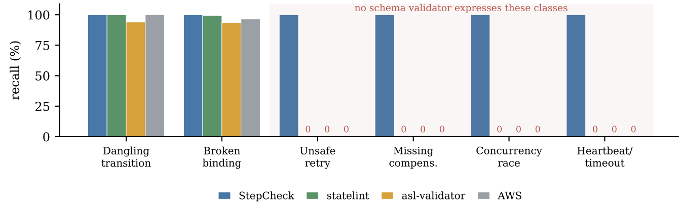
(a) Injected-defect recall (616 mutants)
