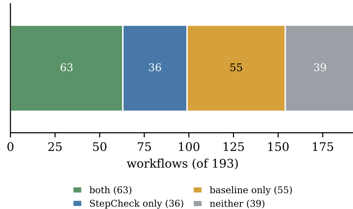
(b) In-the-wild flagged workflows
