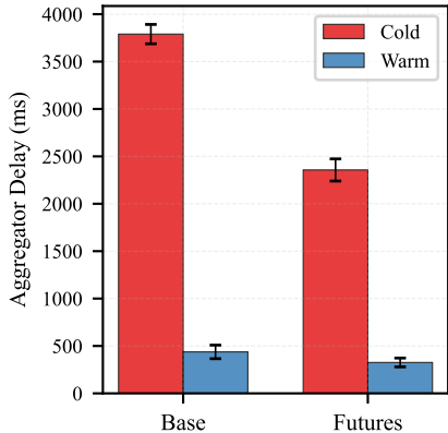
Text Processing
