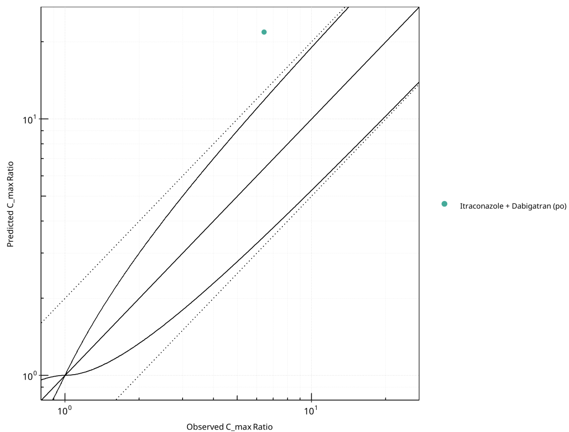
Figure 2-39: Pgp DDI. Victim: Dabigatran. Predicted vs. Observed C max Ratio. ( \delta = 1 in Guest et al. formula)
