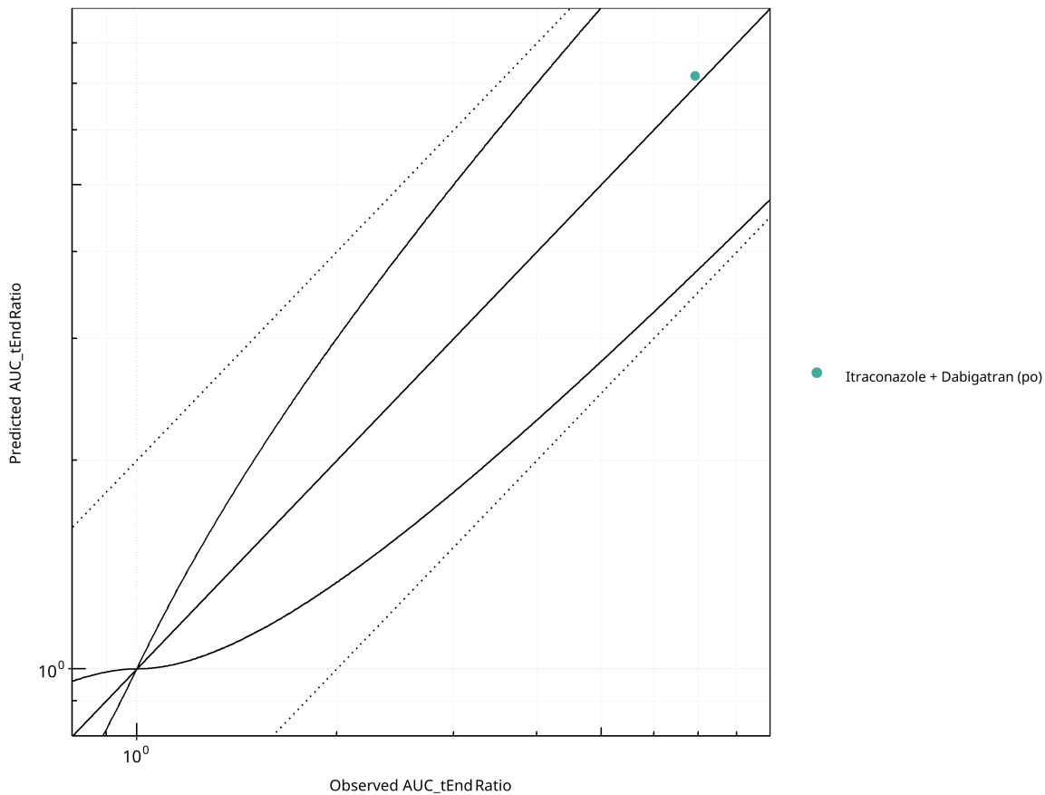
Figure 2-37: Pgp DDI. Victim: Dabigatran. Predicted vs. Observed AUC tEnd Ratio. ( \delta = 1 in Guest et al. formula)
