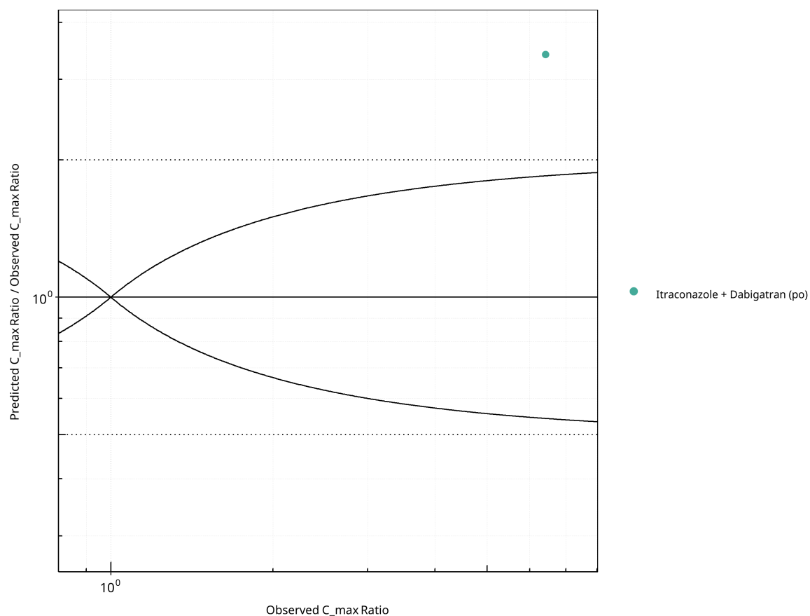
Figure 2-40: Pgp DDI. Victim: Dabigatran. Predicted/Observed vs. Observed C max Ratio. ( \delta = 1 in Guest et al. formula)
