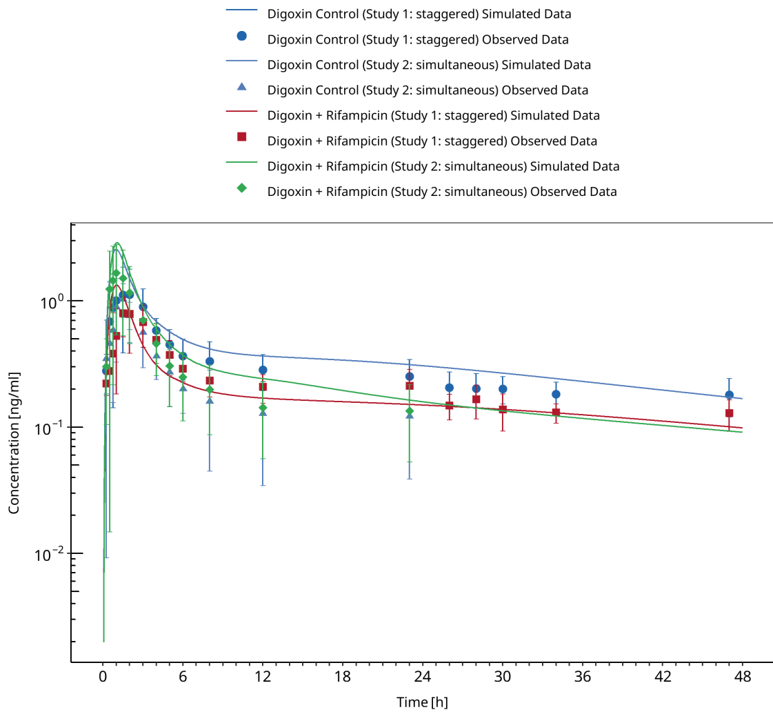
Figure 3-31: Kirby 2012
