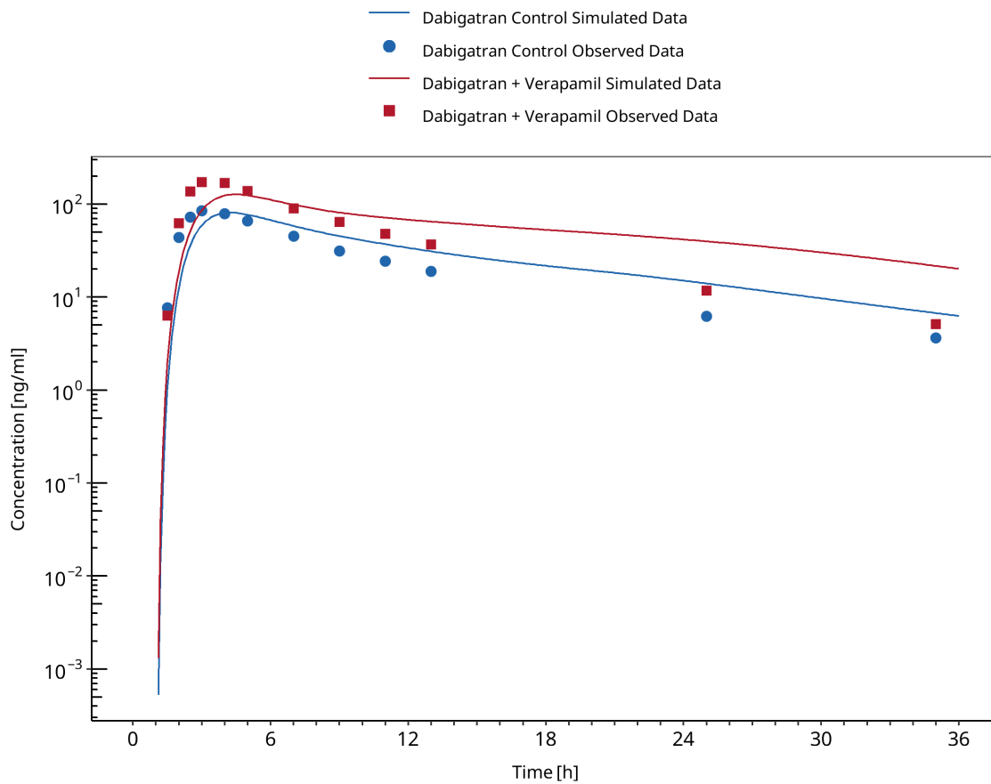
Figure 3-35: Boehringer 1160-0074
