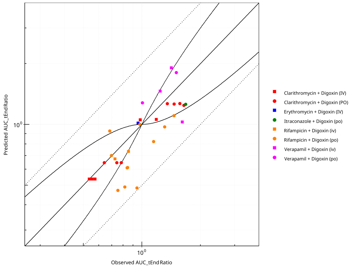
Figure 2-41: Pgp DDI. Victim: Digoxin. Predicted vs. Observed AUC tEnd Ratio. ( \delta = 1 in Guest et al. formula)
