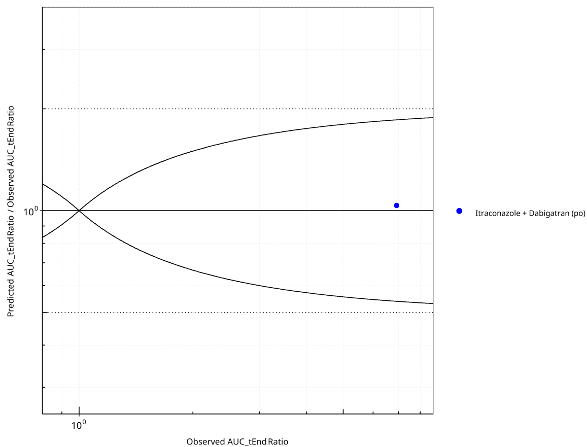
Figure 2-38: Pgp DDI. Victim: Dabigatran. Predicted/Observed vs. Observed AUC_tEnd Ratio. ( \delta = 1 in Guest et al. formula)
