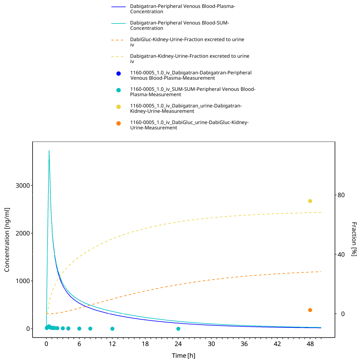
Figure 3-6: 1160-0005 - Dabigatran iv 1.0 mg - lin
