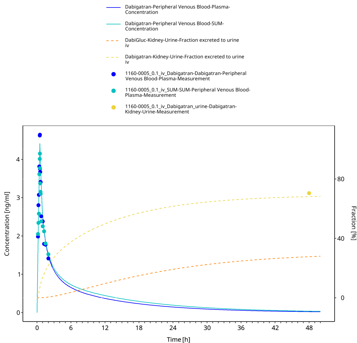
Figure 3-4: 1160-0005 - Dabigatran iv 0.1 mg - lin
