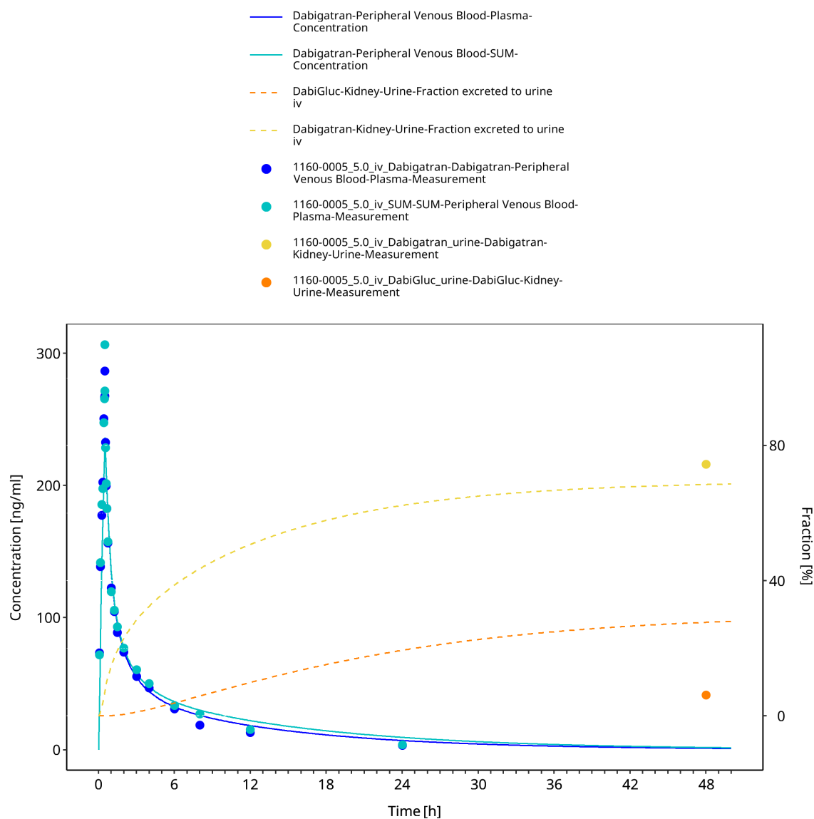
Figure 3-8: 1160-0005 - Dabigatran iv 5.0 mg - lin
