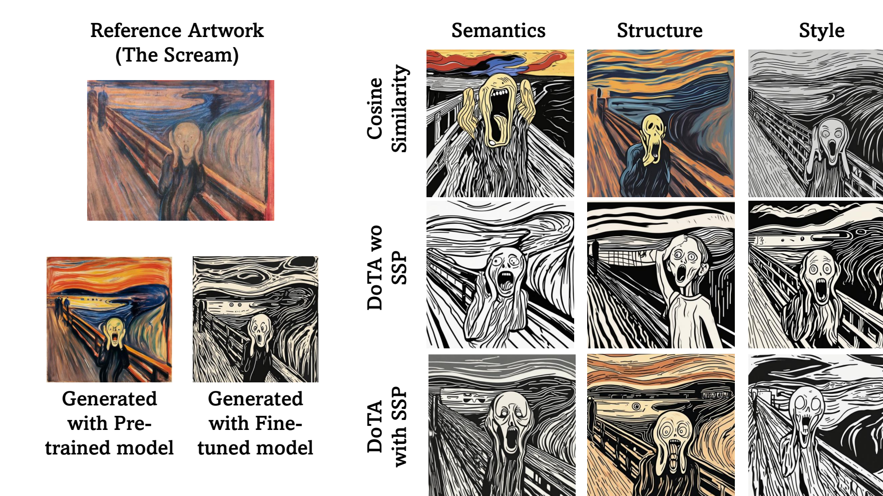
Figure 3: Qualitative comparison of attribution approaches under adversarial attack with different latent representations for the PopArt dataset. We present the images generated for “The Scream” after retraining with Take-K under adversarial attack in different settings. We observe maximum impact of the attack with the cosine similarity based attribution showing drastic changes in semantics, structure, and style in the respective generated images.
