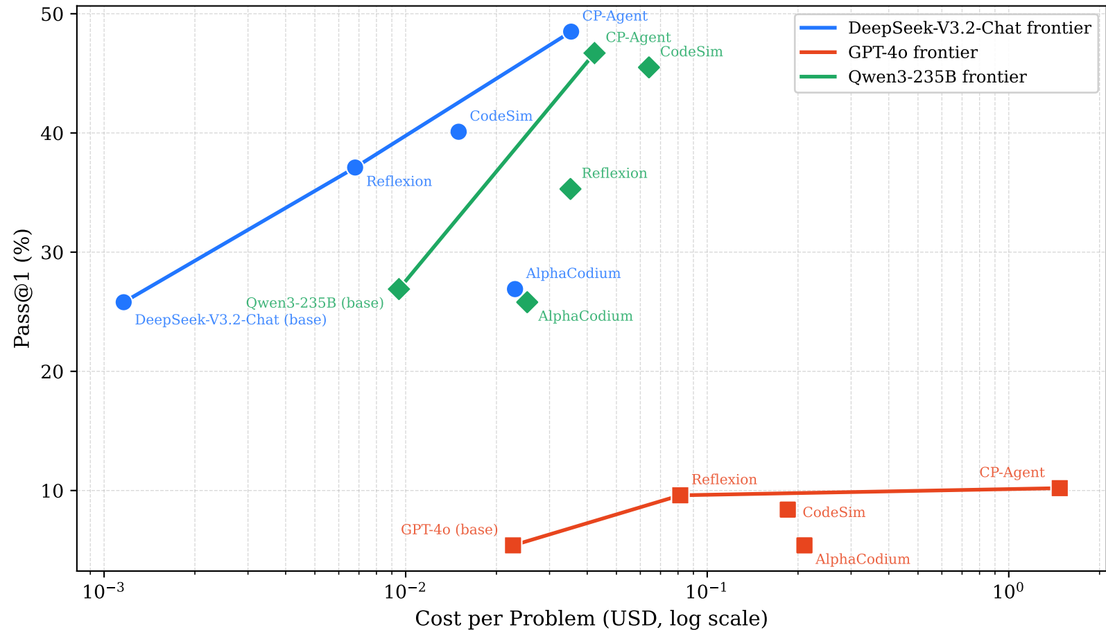
Pass@1 vs. Cost — BCC Efficiency Frontier
