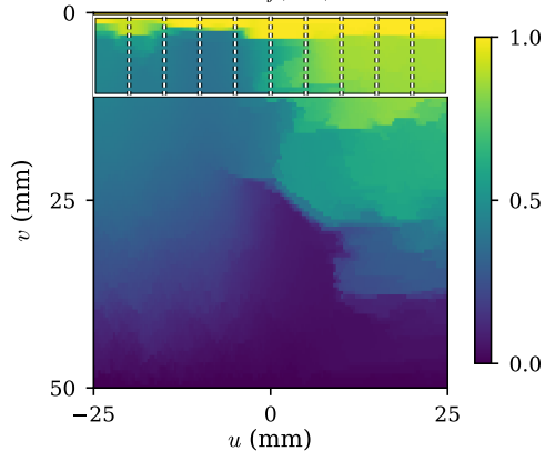
(b) C_j(u, v)
