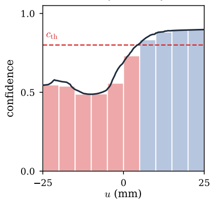
(c) \bar{C}_j(u) and c_j
