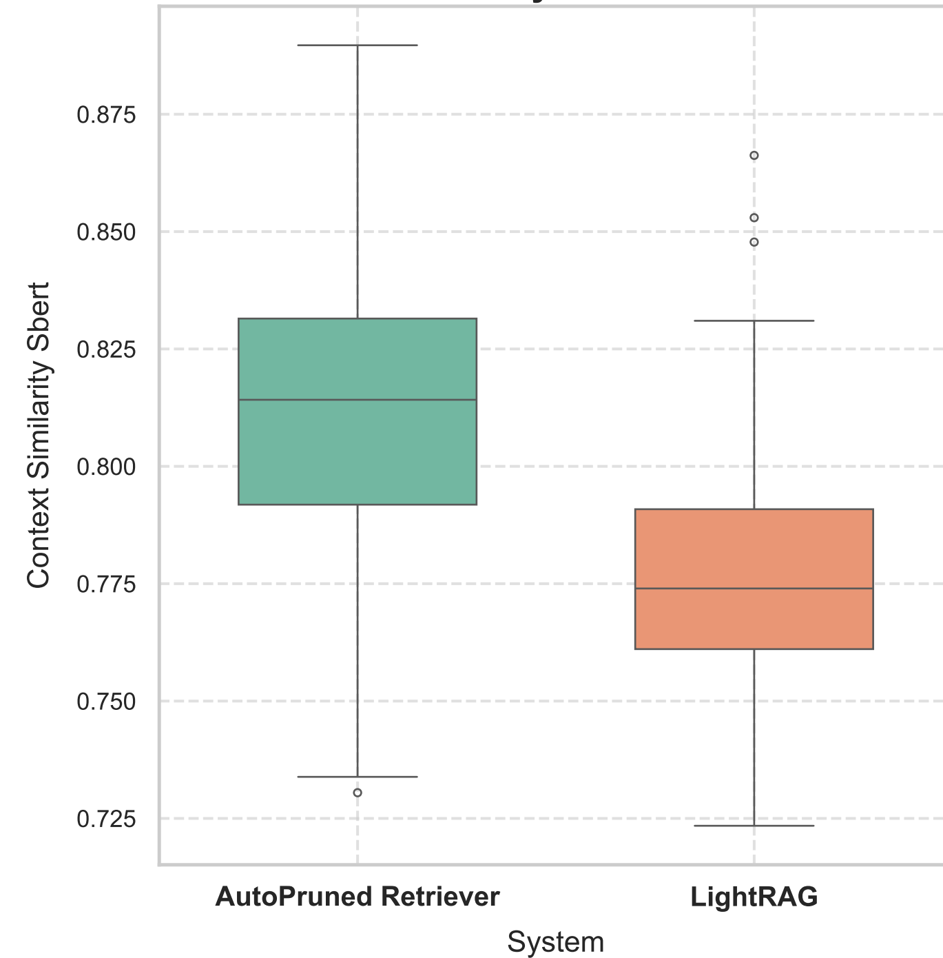
Context Similarity Sbert Distribution
