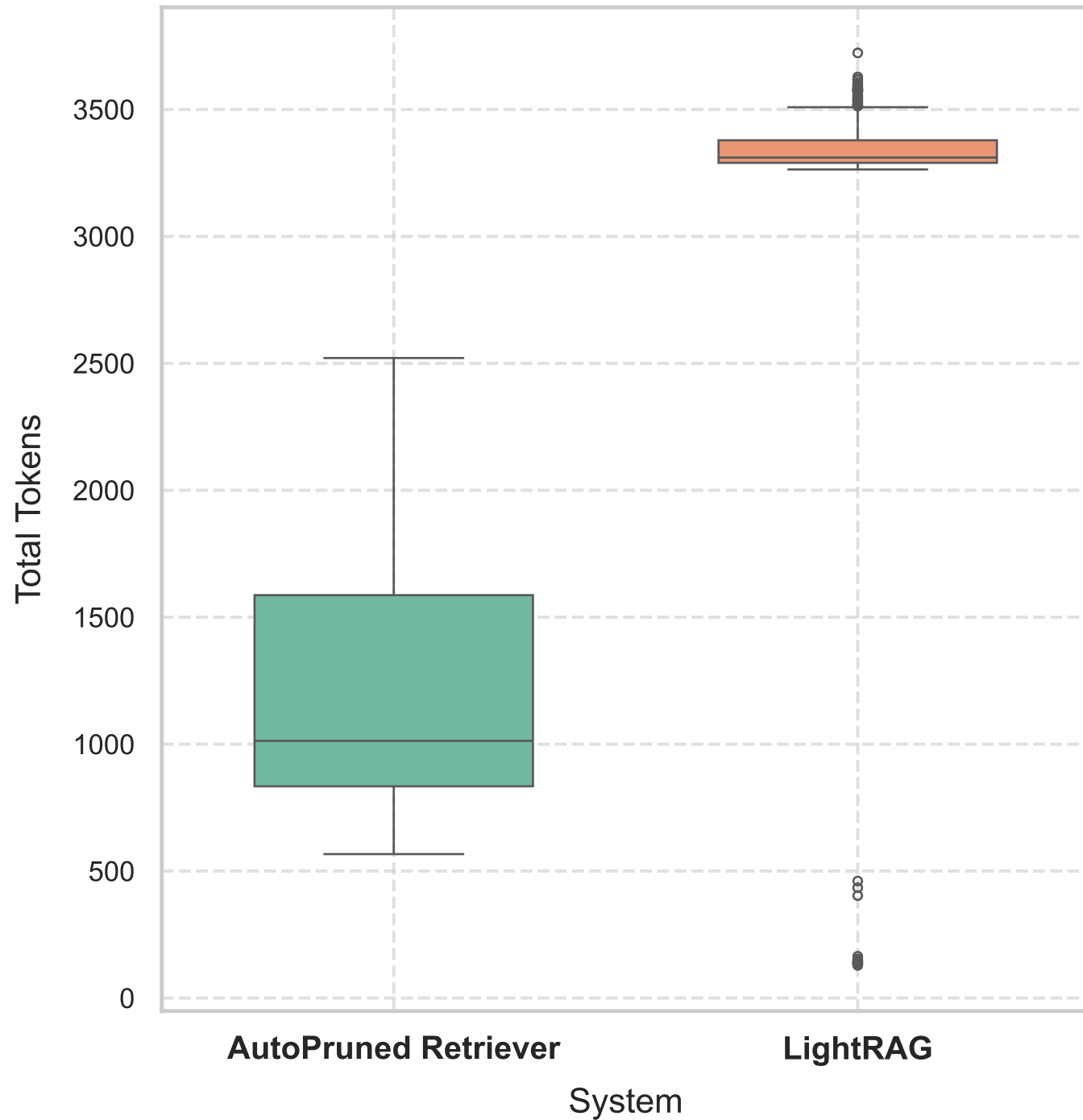
Total Tokens Distribution
