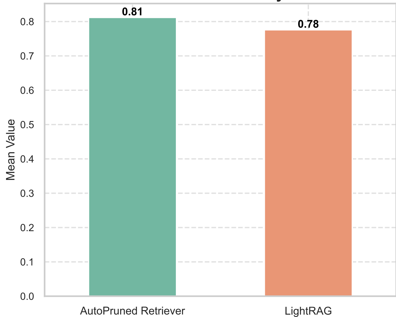
Mean Context Similarity Sbert
