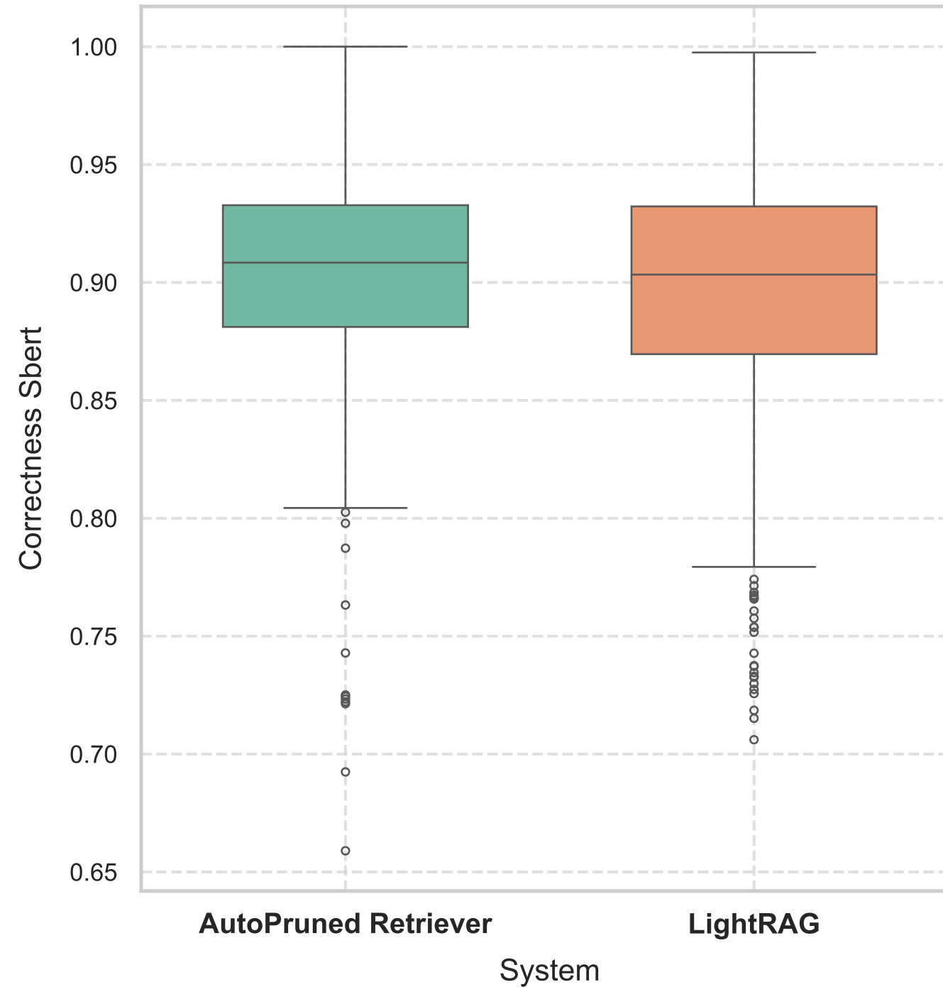
Correctness Sbert Distribution
