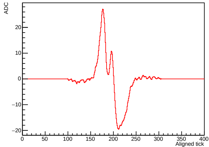
W plane PD - track5_456798
