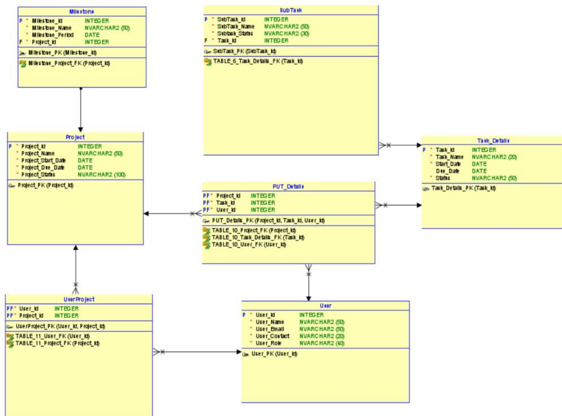
Figure 2 Final ER-Model
